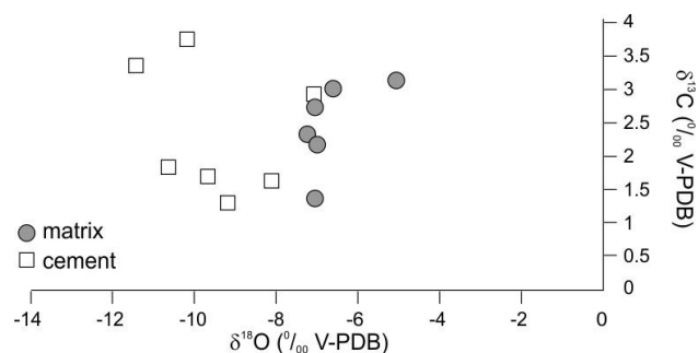
Figure 10. Plot of \delta^{13}\text{C} versus \delta^{18}\text{O} for samples from the La Roche Plissée section.
