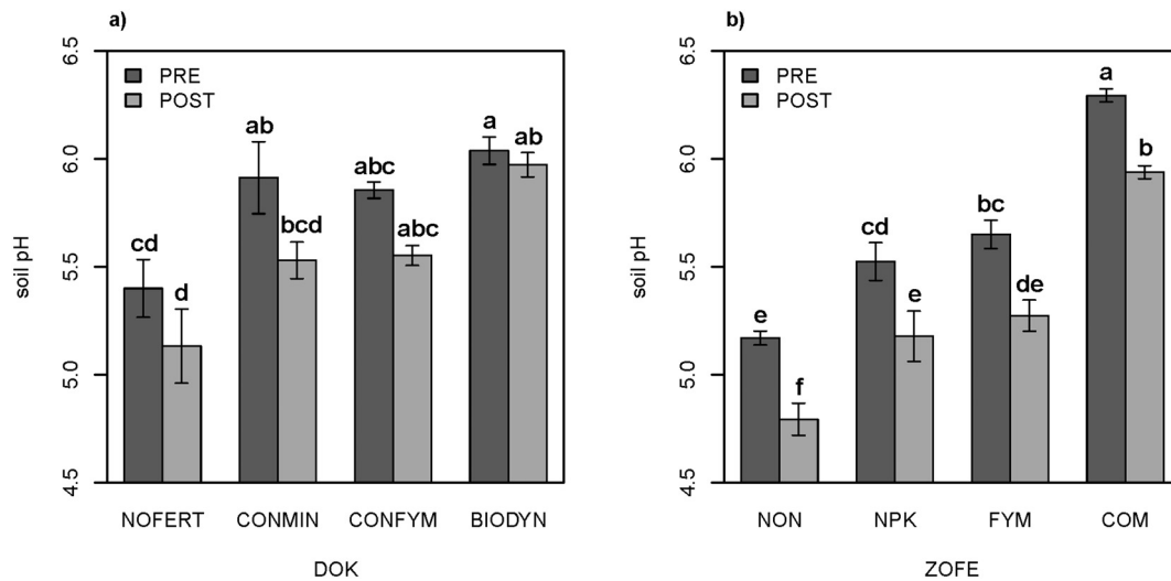
Fig. 1. Soil pH(CaCl 2 ) in the DOK (a) and the ZOFE trial (b) before (PRE) and after (POST) wheat cultivation (mean ± SE, n = 4 (DOK) and n = 5 (ZOFE)). Means with the same letter are not significantly different at p \leq 0.05 according to Tukey multiple comparisons.
