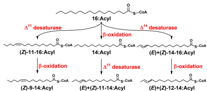
Fig. 2. Pathways toward pheromone precursors in Ostrinia moths. De novo biosynthesis of all precursors starts from palmitoyl-CoA (16:Acyl). A \Delta^{11} desaturase catalyzes the production of (Z)-11-hexadecenoyl [(Z)-11-16:Acyl], which undergoes one cycle of \beta -oxidation to give (Z)-9-tetradecenoyl [(Z)-9-14:Acyl] (9, 51). The same \Delta^{11} desaturase acts on myristoyl-CoA (14:Acyl) to produce (E)- and (Z)-11-tetradecenoyl [(E)+-(Z)-11-14:Acyl] (9, 52). In O. latipennis , a different \Delta^{11} desaturase uniquely catalyzes the stereo-specific production of (E)-11-tetradecenoyl [(E)-11-14:Acyl] (11). Finally, in O. furnacalis , (E)- and (Z)-12-tetradecenoyl [(E)+-(Z)-12-14:Acyl] moieties are produced through chain-shortening of (E)- and (Z)-14-hexadecenoyl [(E)+-(Z)-14-16:Acyl], respectively, the production of which is catalyzed by a \Delta^{14} desaturase (9, 32).
