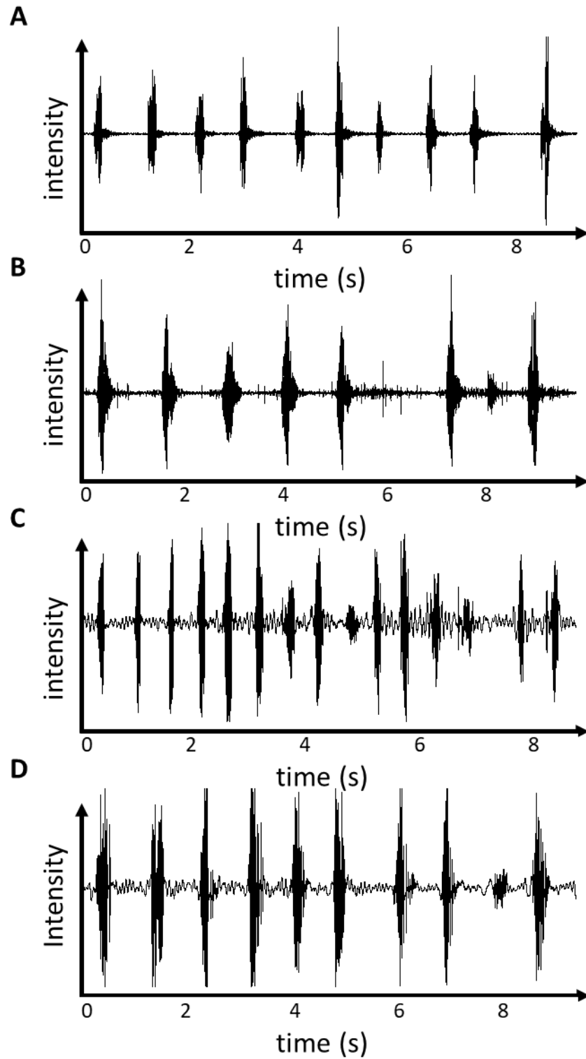
Fig. SP2 Oscillograms of several sounds produced by (A) Hypostomus alatus , (B) H. denticulatus , (C) H. margaritifer and (D) H. strigaticeps .
