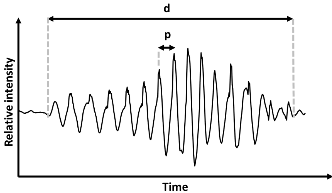
Fig. SP1 Measurements of duration (d) and peak period (p) on a sound.
