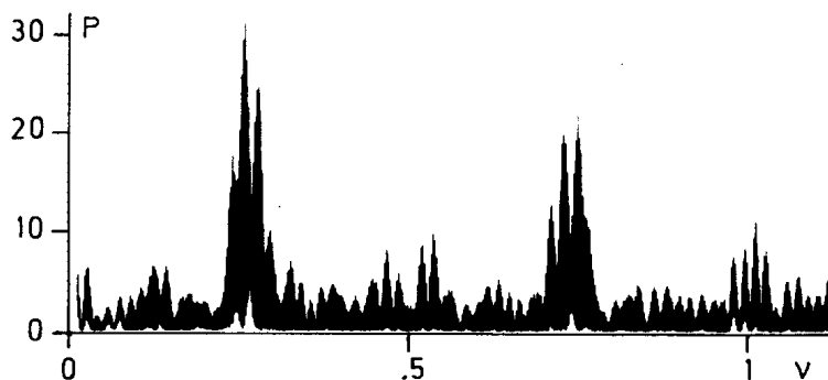
Figure 3: Power spectrum of all observations of HD27563.
