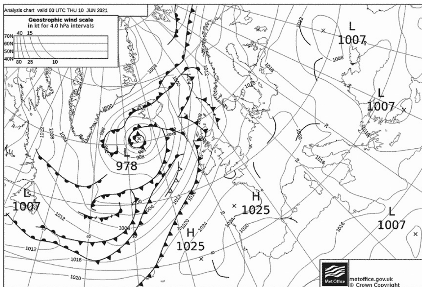
Figure 2. Met Office North Atlantic and European synoptic chart 1 for 0000 UTC on 10 June 2021.
