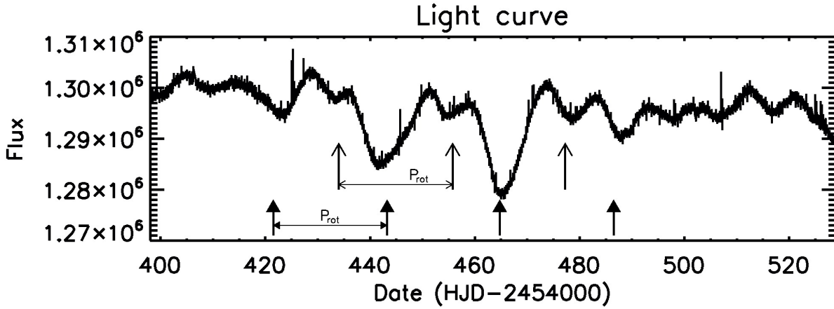
Fig. 1: LC of the target CoRoT-7 without low-frequency filtering. The stellar rotation period, P_{rot} of 23 days can be inferred from spot induced dips, as pointed out by arrows.
