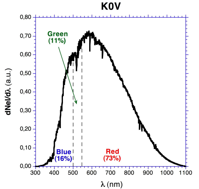
Fig. 10: Distribution of the flux of a K0V star (proxy for CoRoT-7, a G9V star) into the 3 channels, according to the measured relative intensities of the coloured fluxes in photo-electrons.
