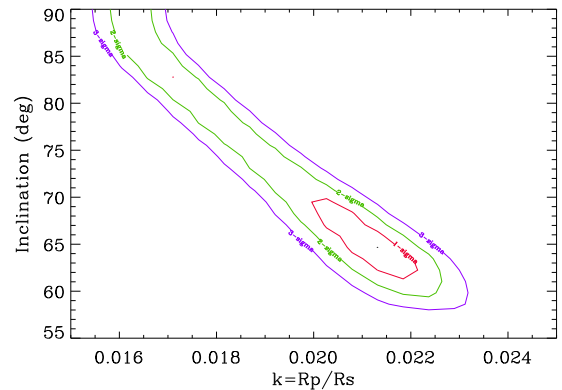
Fig. 18: Contour of the \chi^2 of residuals in the space [relative planet radius, inclination], when a classical fit with 4 free parameters is used, fixing the stellar mass and radius at the spectroscopically determined values. Contours at 68%, 95%, and 99.7% confidence level for parameter estimates are plotted (red, green, and purple contours). One notes the high degeneracy of the secure solutions (green and purple contours).
