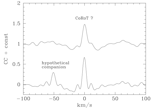
Fig. 13: Top: cross correlation function between the CRIRES spectrum of CoRoT-7 and a synthetic spectrum of an M5V star. Bottom: same as above, but an M5V star spectrum with a shift in RV of -50 km/s was added to the CoRoT-7 spectrum. We conclude that there is no such companion.
