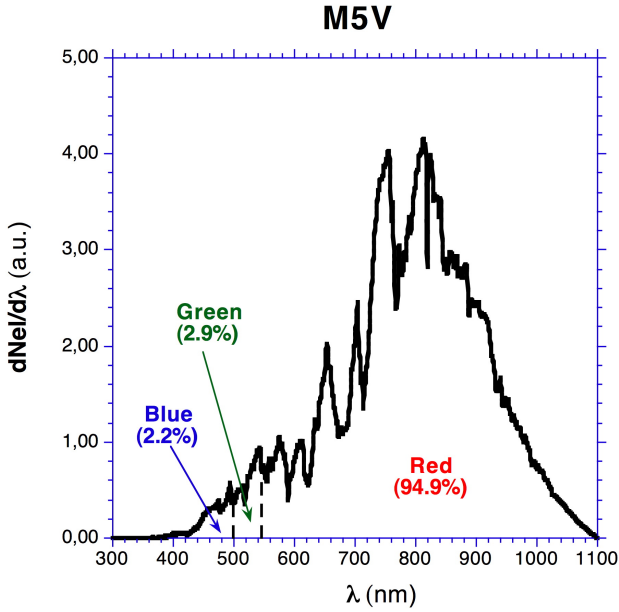
Fig. 11: Expected distribution into the 3 colours of the flux drop, \Delta F , if it was due to the eclipse of a M5V star. Frontiers between colours are the same as in Fig. 10, but the stellar spectrum is different. In that triple system, the flux drop would be significantly redder than observed.
