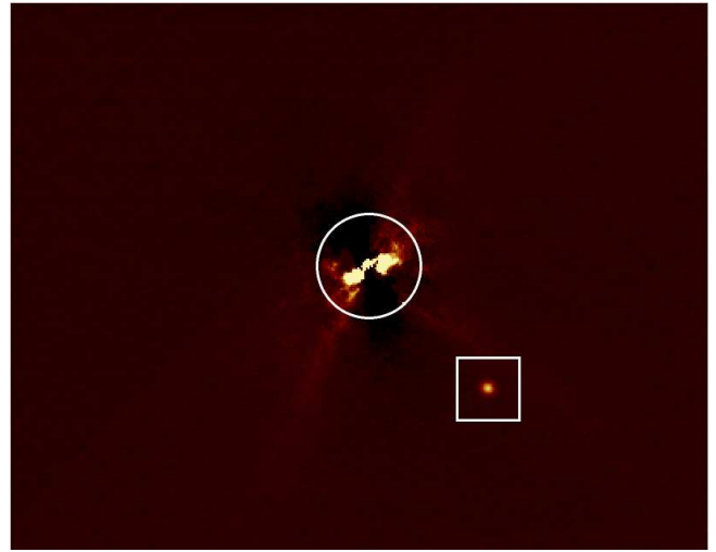
Fig. 8: Central part of the NACO image, after a simulated star 6.5 magnitudes fainter than CoRoT-7 was added (within square). The circle of 400 mas radius defines the only region in which such a star could be confused with residual speckles.
