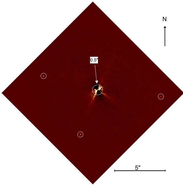
Fig. 7: Final NACO image in J-band after subtraction of a median PSF and de-rotation of the field. The circles locate the three faint stars that are detected in the field, the two at east identified with those marked by arrows in Fig. 6. The scale is given by a line of 5 arcsec length, and the central circle of 0.5 arcsec radius gives an idea of the angular distance at which the presence of a faint star could not be detected close to CoRoT-7. North is at top, and east to the left, as in Fig. 6.
