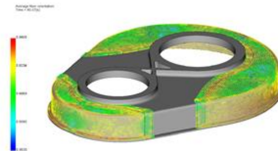
Average fiber orientation
