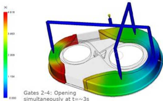
Injection molding of plastic
