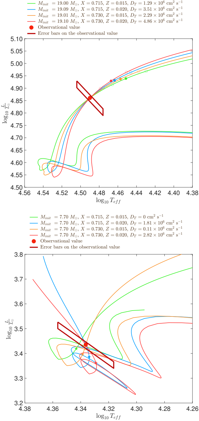
Fig. B.3: Hertzsprung-Russell diagram: evolutionary tracks of Clés models for the primary star ( upper panel ) and secondary star ( lower panel ) corresponding to the best-fit models listed in Table B.1 together with Series II(3) for the primary and Model III S for the secondary. All models have \alpha_{\text{ov}} = 0.30 , primary models have \xi = 1 while secondary models have \xi = 0.1 . The dots over-plotted on the evolutionary tracks of the primary correspond to the models for which k_{2,1} is equal to \bar{k}_2 , while the open circles correspond to the models for which k_{2,1} is equal to \bar{k}_2 \pm \Delta \bar{k}_2 . The filled 5-branch stars over-plotted on the secondary tracks correspond to the models for which the age is equal to the age of the best-fit model of the primary star of same X and Z . The observational value is represented by the red point, and its error bars are represented by the dark red parallelogram.
