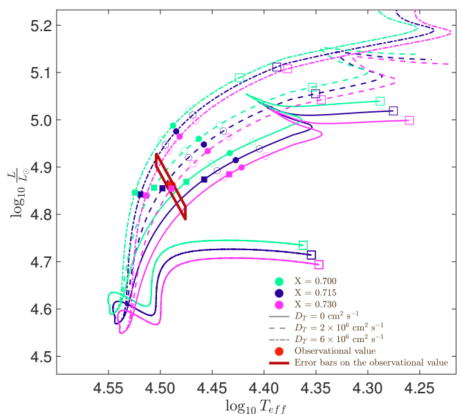
Fig. B.2: Hertzsprung-Russell diagram: evolutionary tracks of Clés models for the primary star having M_{\text{init}} = 19 M_{\odot} , \alpha_{\text{ov}} = 0.30 , \xi = 1 , Z = 0.015 , X = 0.700 (water green), 0.715 (dark blue), and 0.730 (pink), and D_T = 0 \text{ cm}^2 \text{ s}^{-1} (solid line), 2 \times 10^6 \text{ cm}^2 \text{ s}^{-1} (dashed line), 6 \times 10^6 \text{ cm}^2 \text{ s}^{-1} (dotted-dashed line), and 10 \times 10^6 \text{ cm}^2 \text{ s}^{-1} (dotted line). The dots over-plotted on the corresponding tracks correspond to the models for which k_{2,1} is equal to \bar{k}_2 , while the open circles correspond to the models for which k_{2,1} is equal to \bar{k}_2 \pm \Delta \bar{k}_2 . The filled and open squares over-plotted on the tracks correspond to the models for which the mass is equal to the observed value within the error bars. The observational value is represented by the red point, and its error bars are represented by the dark red parallelogram.
