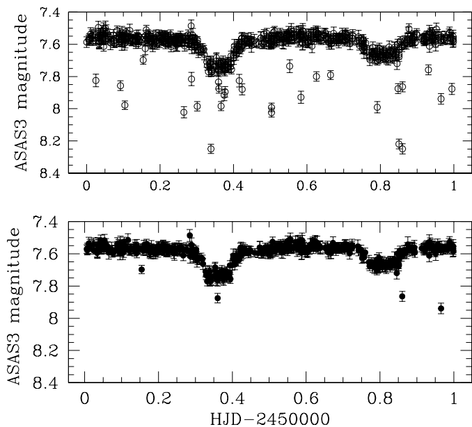
Fig. 1: ASAS-3 lightcurve phase-folded using the orbital period given in Table 3. The top panel illustrates the initial ASAS-3 data set, whilst the bottom panel shows the data after the 1.25\sigma clipping.
