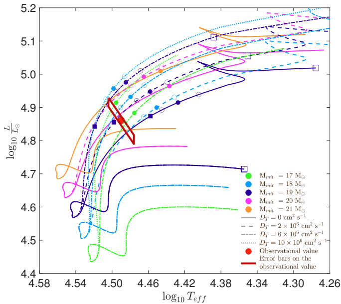
Fig. 18: Hertzsprung-Russell diagram: evolutionary tracks of Clés models for the primary star of M_{\text{init}} = 17 M_{\odot} (green), 18 M_{\odot} (light blue), 19 M_{\odot} (dark blue), 20 M_{\odot} (pink), and 21 M_{\odot} (orange), and D_T = 0 \text{ cm}^2 \text{ s}^{-1} (solid line), 2 \times 10^6 \text{ cm}^2 \text{ s}^{-1} (dashed line), 6 \times 10^6 \text{ cm}^2 \text{ s}^{-1} (dotted-dashed line), and 10 \times 10^6 \text{ cm}^2 \text{ s}^{-1} (dotted line). All models have \alpha_{\text{ov}} = 0.30 and \xi = 1 . The dots over-plotted on the corresponding tracks correspond to the models for which k_{2,1} is equal to \bar{k}_2 , while the open circles correspond to the models for which k_{2,1} is equal to \bar{k}_2 \pm \Delta \bar{k}_2 . The filled and open squares over-plotted on the tracks having an initial mass of 19 M_{\odot} correspond to the models for which the mass equals the observational value within the error bars. The observational value is represented by the red point, and its error bars are represented by the dark red parallelogram.
