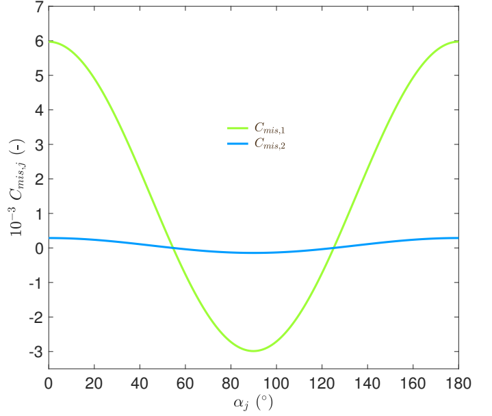
Fig. 20: Behaviour of C_{\text{mis},1} and C_{\text{mis},2} as a function of \alpha_1 and \alpha_2 , the angle between the primary and secondary stellar rotation axis, respectively, and the normal to the orbital plane.
