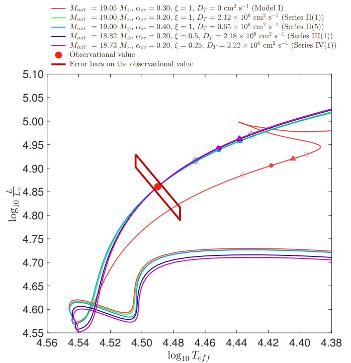
Fig. 16: Hertzsprung-Russell diagram: evolutionary tracks of Clés models corresponding to the following best-fit models: Model I (coral), Series II(1) (green), Series II(5) (light blue), Series III(1) (dark blue), and Series IV(1) (plum). The dots and triangles over-plotted on the corresponding tracks correspond to the models for which k_{2,1} is equal to \bar{k}_2 and 0.00139, respectively, while the open circles correspond to the models for which k_{2,1} is equal to \bar{k}_2 \pm \Delta k_2 . The observational value is represented by the red point, and its error bars are represented by the dark red parallelogram.
