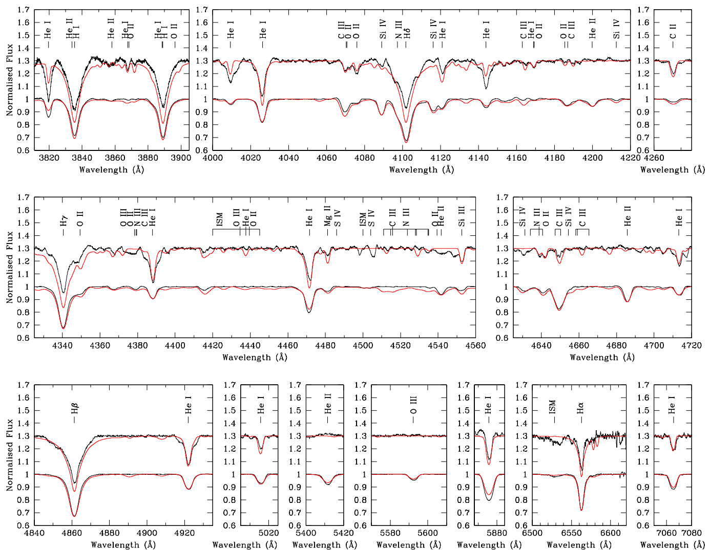
Fig. 5: Normalised disentangled spectra (in black) of the primary and secondary star of HD 152219 (note that the spectrum of the secondary star is shifted by +0.3 in the y-axis for convenience) together with the respective best-fit CMFGEN model atmosphere (in red).
