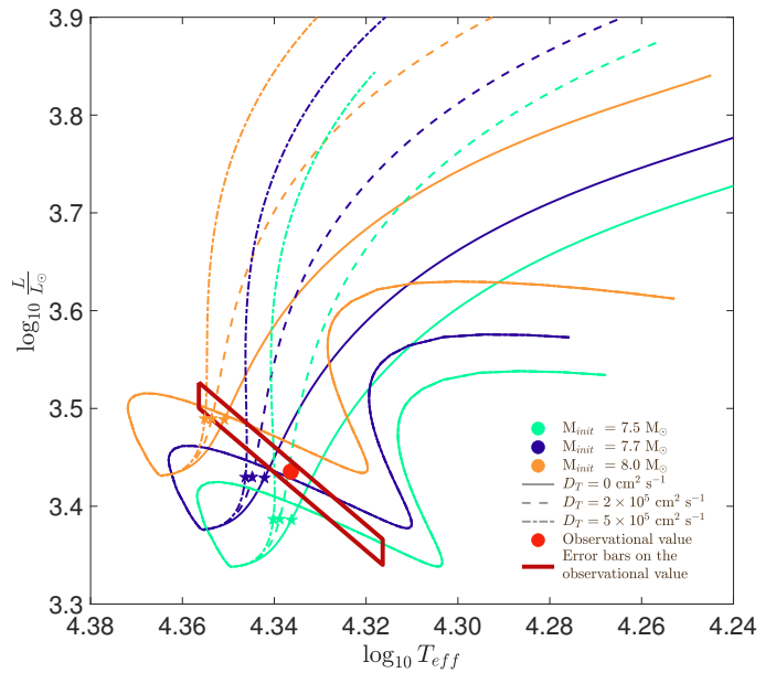
Fig. 19: Hertzsprung-Russell diagram: evolutionary tracks of Clés models for the secondary star of M_{\text{init}} = 7.5 M_{\odot} (water green), 7.7 M_{\odot} (dark blue), and 8.0 M_{\odot} (orange), and D_T = 0 \text{ cm}^2 \text{ s}^{-1} (solid line), 2 \times 10^5 \text{ cm}^2 \text{ s}^{-1} (dashed line), and 5 \times 10^5 \text{ cm}^2 \text{ s}^{-1} (dotted-dashed line). All models have \alpha_{\text{ov}} = 0.30 and \xi = 0.1 . The filled 5-branch stars over-plotted on the tracks correspond to the models for which the age is equal to the age of the best-fit models of the primary star (i.e. about 9 Myr). The observational value is represented by the red point, and its error bars are represented by the dark red parallelogram.
