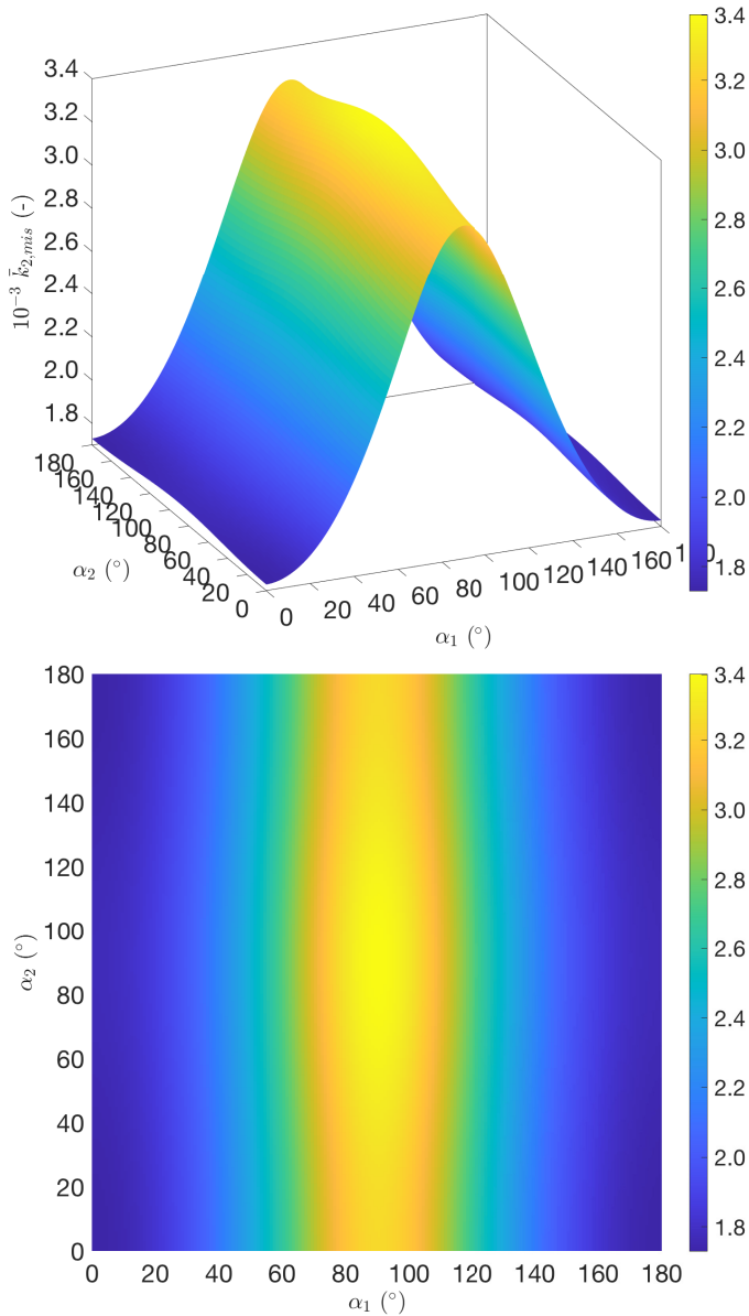
Fig. 21: Behaviour of \bar{k}_{2,\text{mis}} as a function of \alpha_1 and \alpha_2 , the angle between the primary and secondary stellar rotation axis, respectively, and the normal to the orbital plane.
