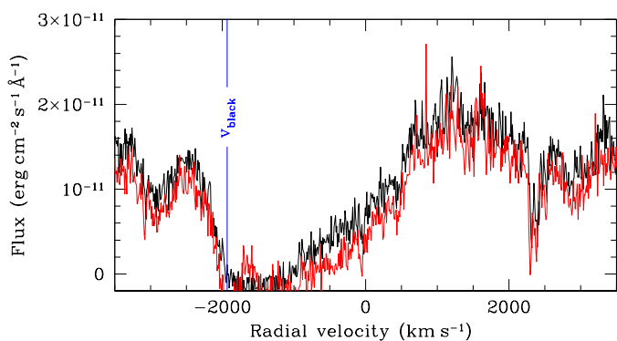
Fig. 4: Determination of v_{\text{black}} on the absorption trough of C IV \lambda\lambda 1548, 1551 as observed in the IUE spectra of HD 152219. The black and red curves correspond to observations SWP 56939 and SWP 56953, respectively.
