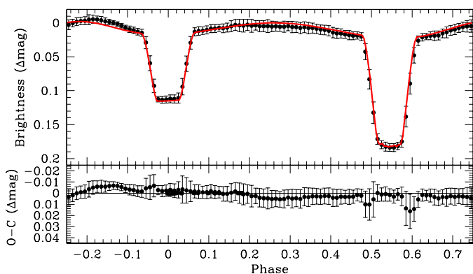
Fig. 10: Upper panel : best-fit Nightfall solution of the TESS-39 light curve of HD 152219. Lower panel : residuals over the best-fit solution.
