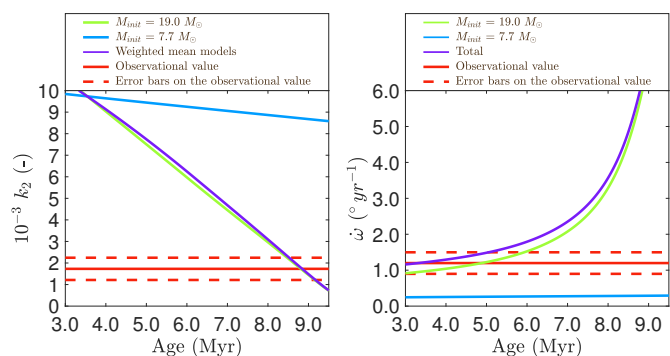
Fig. 13: Left panel : Evolution as a function of stellar age of the internal structure constant (to which the empirical correction Eq. (22) has been applied) for Clés models with initial mass of 19.0 M_{\odot} and \xi = 1 ( k_{2,1} , green) and initial mass of 7.7 M_{\odot} and \xi = 0.1 ( k_{2,2} , blue), both models have \alpha_{\text{ov}} = 0.30 and no turbulent diffusion. The weighted-average mean of the k_2 -values, computed using Eq. (19), is also depicted ( \bar{k}_2 , purple). Right panel : Evolution as a function of stellar age of the total apsidal motion rate (purple) and of the contributions of the two stars (green and blue). The observational value of the corresponding parameter and its error bars are represented by the solid red line and the dashed red horizontal lines, respectively.
