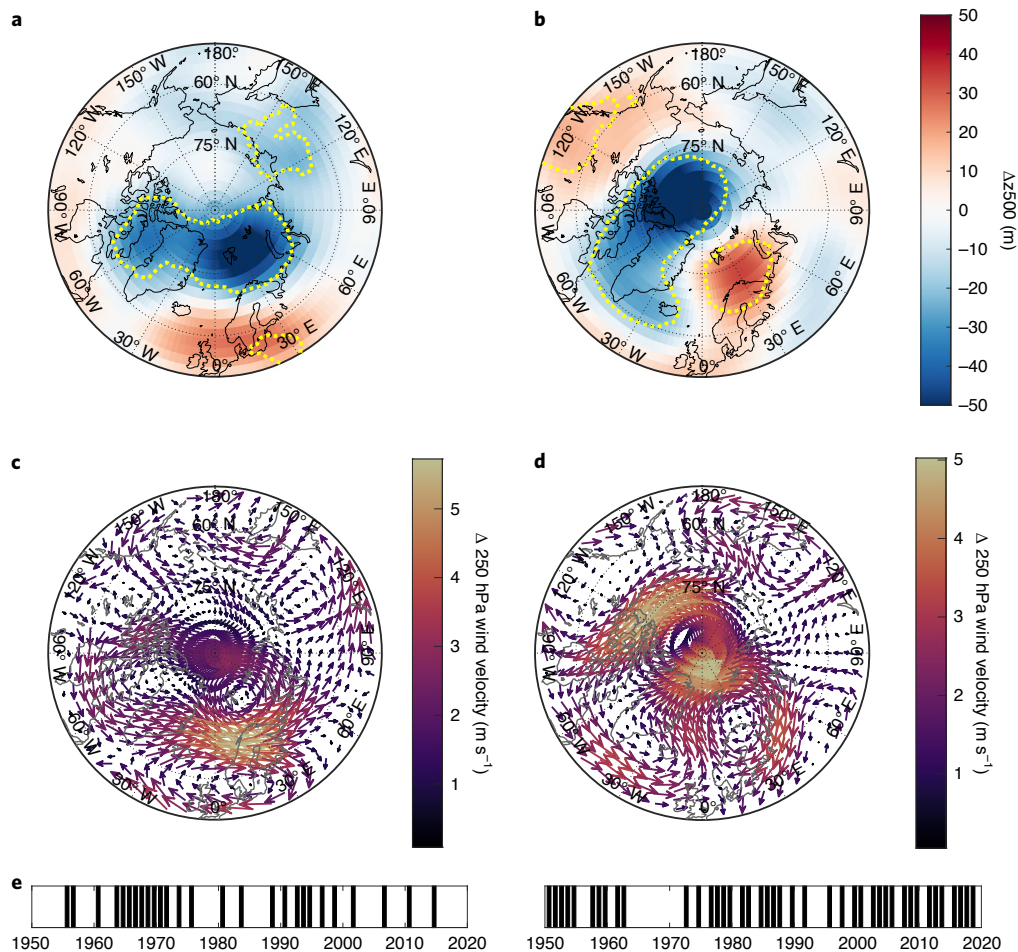
Fig. 5 | Composites of selected atmospheric variables in years belonging to an identified mass-balance category. a, JJA mean of the z500 of all detrended (order n=3 ) positive mass-balance years minus all negative years of the study period. b, Same as a but for all years with positive mass-balance anomalies in ACN while negative in SVA minus all years with signs reversed. Areas of significance ( P < 0.05 ) are contained within yellow dotted contours. c,d, Same as a,b , respectively, but showing the differences of wind velocity and direction at 250 hPa (jet-stream level). Analyses are based on reanalysis data (Methods). e, The mass-balance years (MAR3.11 SMB) contained in the preceding respective composites (black). Composites for each of the four categories are shown in Extended Data Figs. 8 and 9. Uncertainties in the z500 composites arising from uncertainties in the SMB reconstruction and the inferred categorization are presented in Extended Data Fig. 10.
