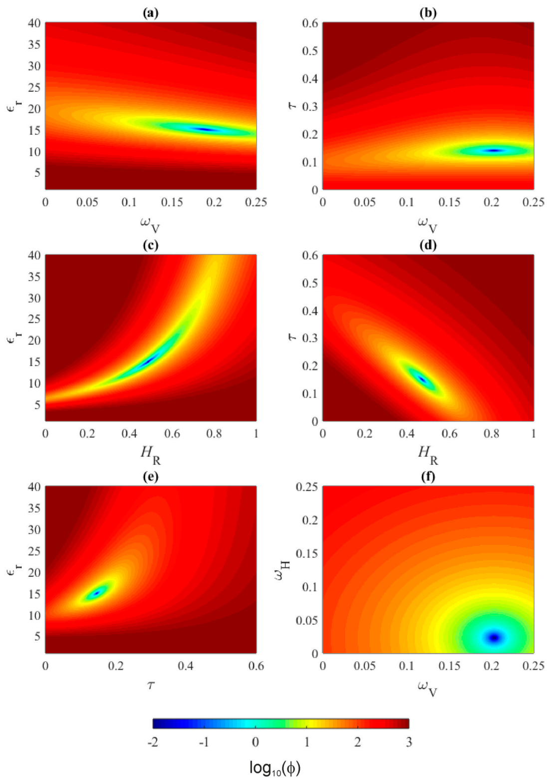
Figure 11. Response surfaces of the logarithm of the objective function ( \log_{10}(\phi) ) in the following parameter planes: \epsilon_T - \omega_V (a); \tau - \omega_V (b); \epsilon_T - H_R (c); \tau - H_R (d); \epsilon_T - \tau (e); and \omega_H - \omega_V (f).
