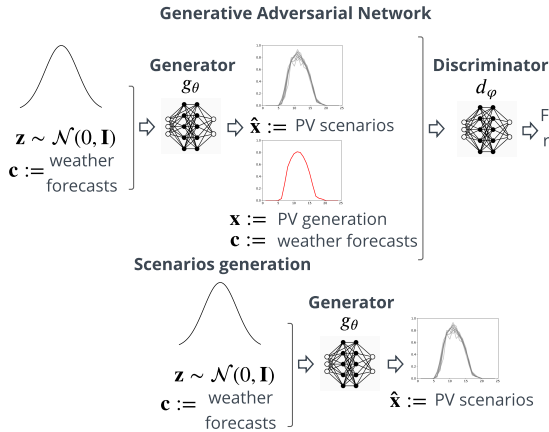
Figure 5: The process of the conditional generative adversarial network is illustrated for PV generation.
