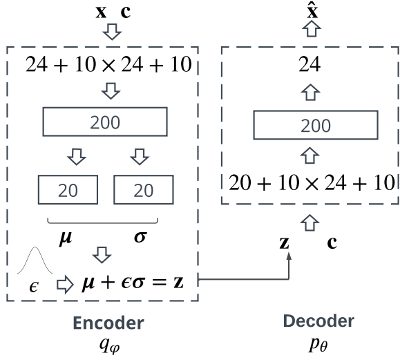
Figure B.12: Variational autoencoder structure implemented for the wind dataset.
