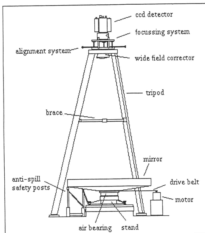
Figure 2. Entire liquid mirror telescope system.
