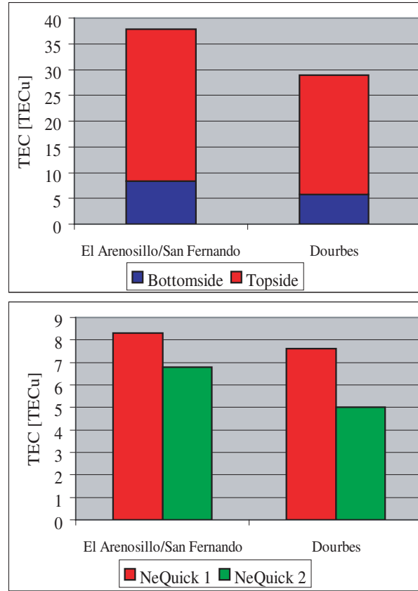
Fig. 6. Proportion of TEC within bottomside and topside (top) and yearly topside TEC standard deviation (bottom)
