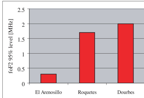
Fig. 2. Influence of ionosonde scaling validation on f_oF_2
