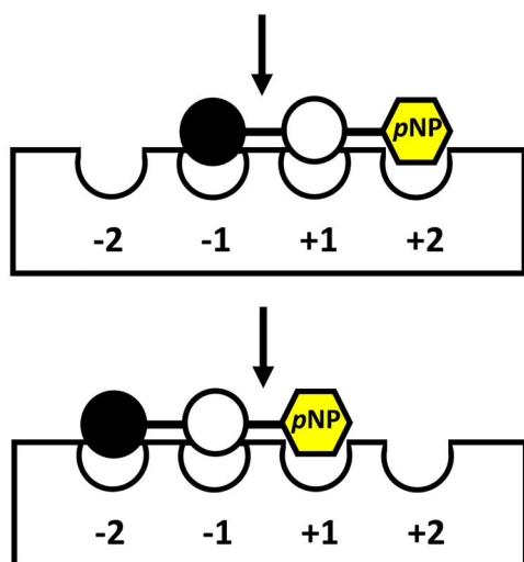
Fig. 4. Binding of G2- pNP in the Amyrel active site. Subsites are numbered with respect to the cleavage site (arrow). Closed circle, nonreducing end of the substrate; open circle, glucopyranose unit. Upper panel: binding mode resulting in G1 + G1- pNP release. Lower panel: binding mode resulting in G2 + pNP release. Only subsites required for G2- pNP binding are depicted.
