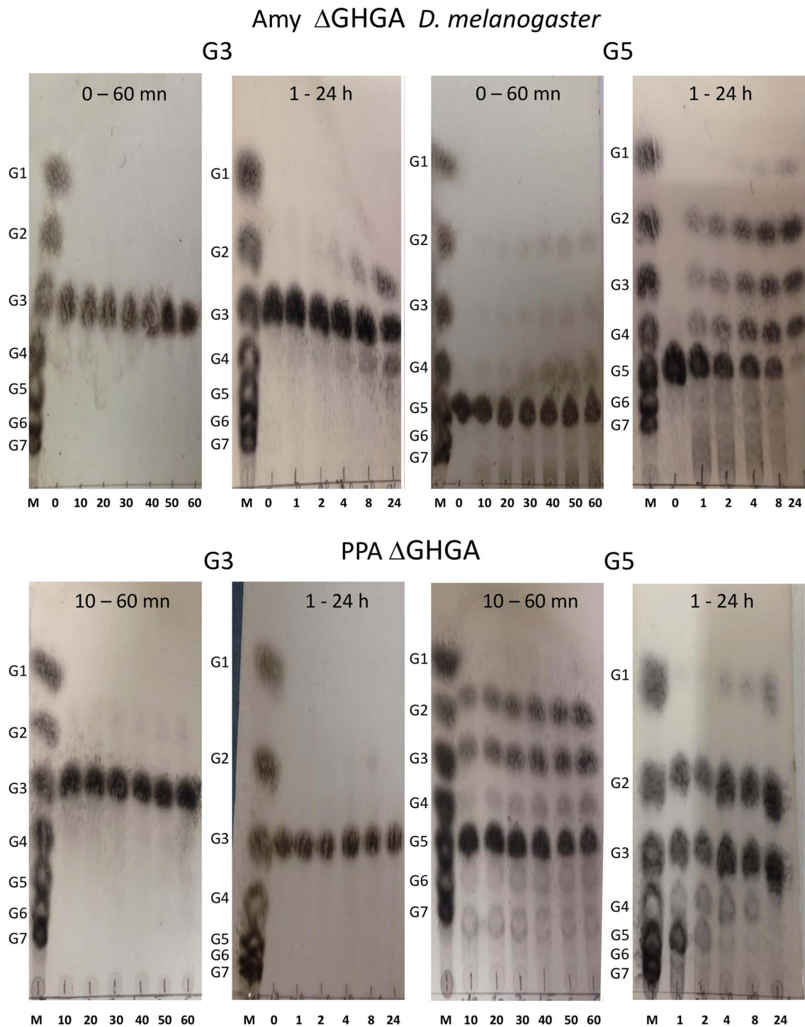
Fig. 6. TLC of reaction time courses of maltooligosaccharides G3 and G5 (5 mg/mL) digested by the mutants Amy \Delta GHGA (upper panel, 20 nM) and PPA \Delta GHGA (lower panel, 140 nM). Note the disproportionation of G3 by Amy \Delta GHGA as well as the appearance of G1 and of multiple maltooligosaccharides with G5 as substrate for both mutants. M, maltooligosaccharide ladder. Reaction times are indicated in minutes and hours.
