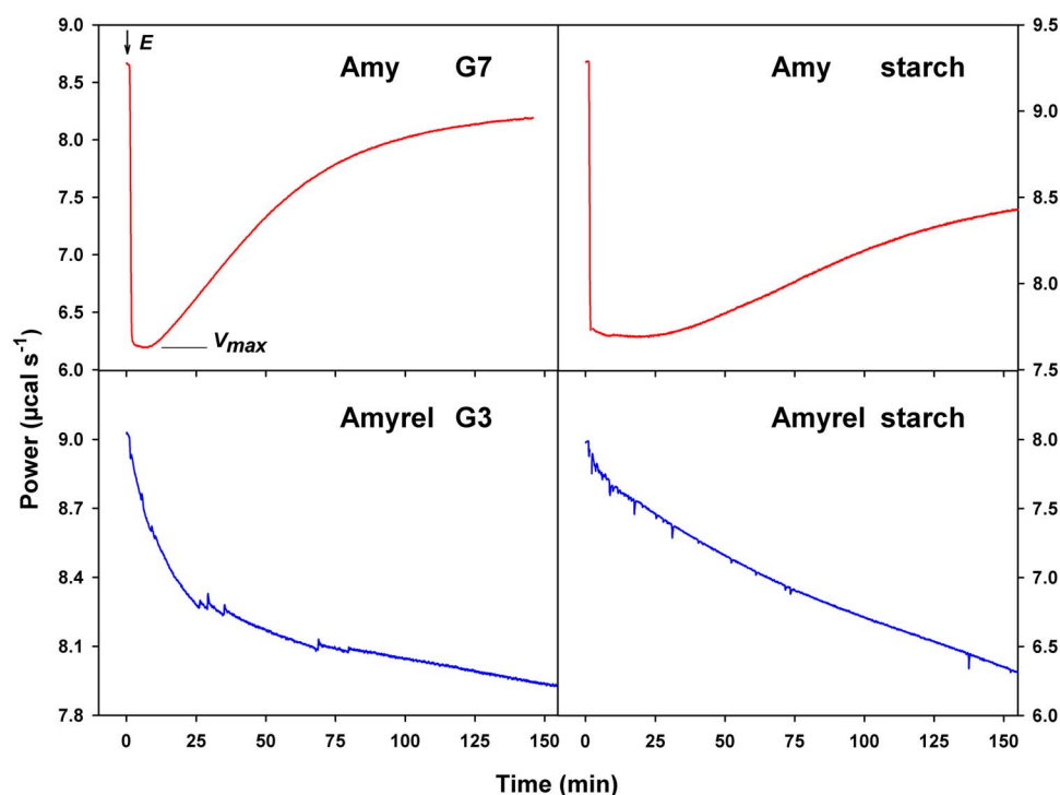
Fig. 5. Reaction time courses of Amy and Amyrel on polysaccharides recorded by ITC. The records start with the injection (arrow) of enzyme (E) in the reaction vessel. For Amy, the heat release of \alpha -(1–4) hydrolysis reaches a steady state ( V_{max} ) allowing the k_{cat} determination. For Amyrel, a steady state is not reached, indicating a competing reaction with opposite enthalpy, attributed to \alpha -(1–4) bond synthesis.
