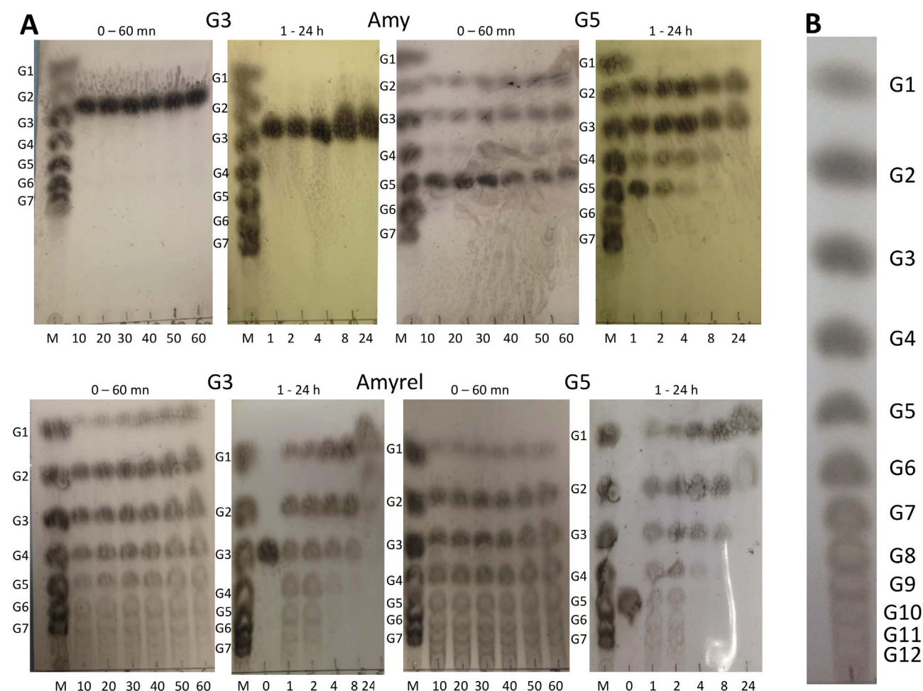
Fig. 2. (A) TLC of reaction time courses of maltooligosaccharides G3 and G5 (5 mg/mL) digested by the Amy \alpha -amylase (upper panel) and Amyrel (lower panel) from D. melanogaster . Final concentration of enzymes: 6 nM Amy, 150 nM Amyrel. M, maltooligosaccharide ladder. Reaction times are indicated in minutes and hours. (B) Typical TLC pattern of maltooligosaccharides produced by Amyrel (450 nM) with G3 (20 mg/mL) as substrate after 30-min incubation. Maltooligosaccharides are numbered up to the last detectable product.
