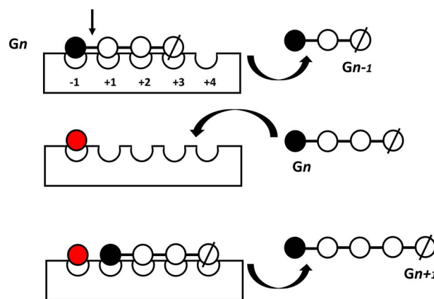
Fig. 7. Disproportionation reaction of maltooligosaccharides by Amyrel, illustrated for G4. Subsites are numbered with respect to the cleavage site (arrow). Closed circle, nonreducing end; open circle, glucopyranose unit; open slashed circle, reducing end; in red, the covalent glucosyl-enzyme intermediate. For details, see text. Only subsites required for G4 binding are depicted.
