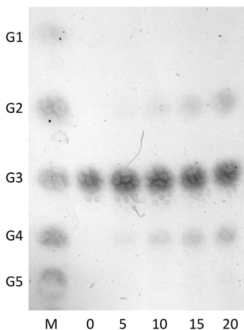
Fig. 3. Disproportionation of maltooligosaccharides by Amyrel. TLC of the reaction time course by Amyrel (35 nM) with G3 (5 mM) as substrate showing the appearance of the first products G_{n-1} and G_{n+1} . M, maltooligosaccharide ladder. Reaction times are indicated in minutes.
