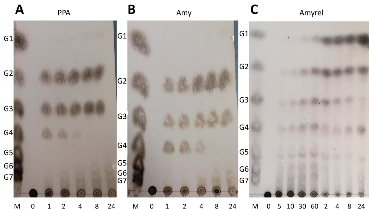
Fig. 1. TLC of reaction time courses of soluble starch (5 mg/mL) digested by (A) PPA, (B) Amy \alpha -amylase from D. melanogaster and (C) Amyrel from D. melanogaster . Final concentration of enzymes: 15 nM PPA, 6 nM Amy, 150 nM Amyrel. M, maltooligosaccharide ladder. Reaction times are indicated in hours (A, B) and in minutes and hours (C).
