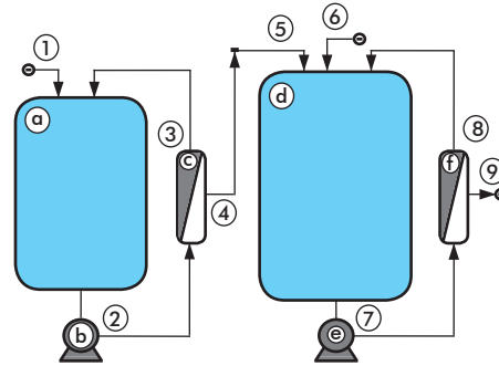
Figure 2. Two-stage continuous-perfusion cell culture system for MAb production in hybridoma cells. a) First bioreactor, stage 1. b) First circulation pump. c) First cell separator and flow splitter. d) Second bioreactor, stage 2. e) Second circulation pump. f) Second cell separator and flow splitter. Numbered arrows represent connecting flows.
