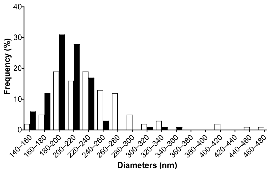
Figure 2. Size distribution of the fiber diameter for chitosan membrane in white and curdlan–chitosan membrane in black measured by image analysis with ImageJ on 100 randomly selected fibers.
