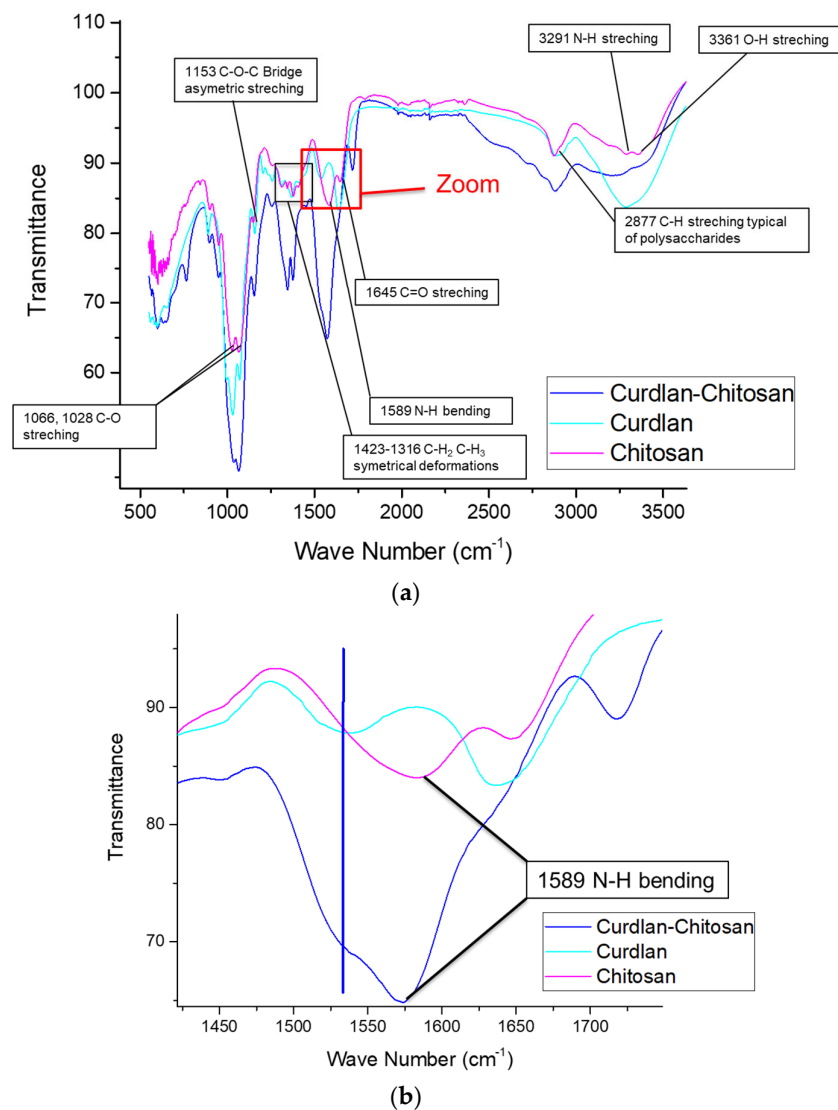
Figure 3. ATR-FTIR spectra of curdlan and chitosan starting polymers and of the curdlan–chitosan fibers. (a) The full spectrum with peaks attribution [51]. (b) Zoom on the 1400 to 1700\text{ cm}^{-1} spectral range to identify characteristic peaks of both curdlan and chitosan of the blend spectrum (blue line denotes the 1530\text{ cm}^{-1} band specific to curdlan).
