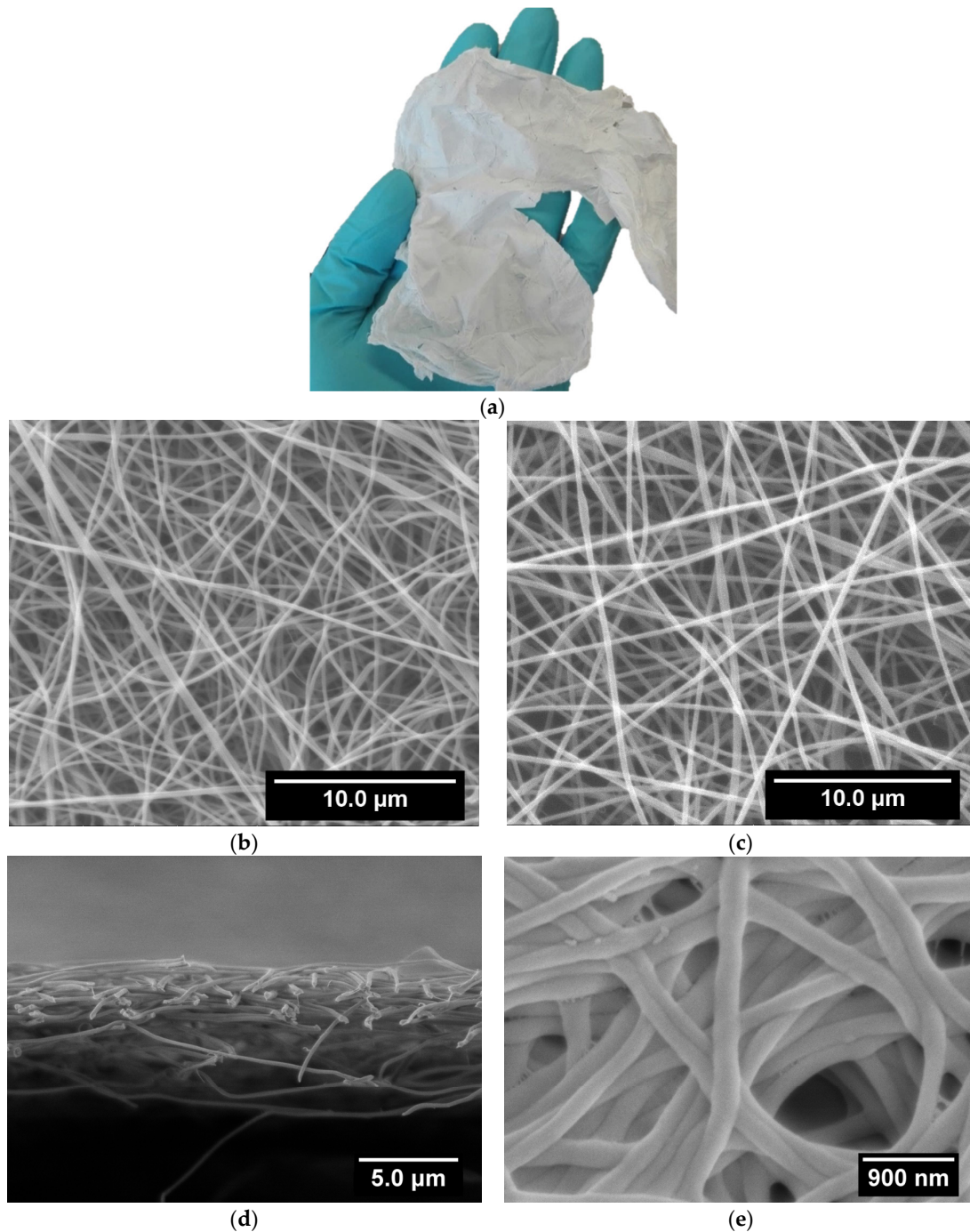
Figure 1. (a) Photography of the macroscopic aspect of the curdlan–chitosan scaffold as removed from the collector and SEM images of (b) electrospun chitosan membrane (Acceleration Voltage (AV) 20 keV), (c) electrospun curdlan–chitosan membrane (AV 20 keV), (d) cross section of electrospun curdlan–chitosan membrane (AV 3 keV), (e) electrospun curdlan–chitosan membrane after stabilization (AV 3 keV).
