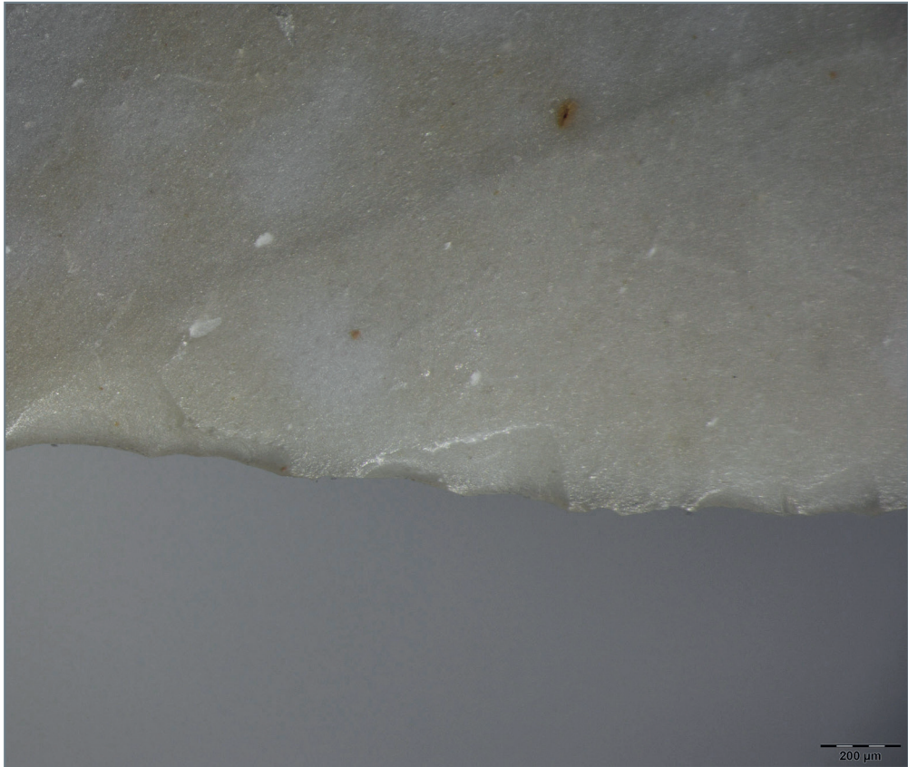
Fig. 9: Bending-initiated, partly obliquely oriented scarring on RM 5 (Jurassic chert), used for cutting soft leather for 12 minutes. The lighting has been adjusted in the image editing software to enhance the visibility of the scars and the chert therefore appears darker than it is in reality. Original magnification 40×, scale bar 200 µm (photo: N. Taipale).
