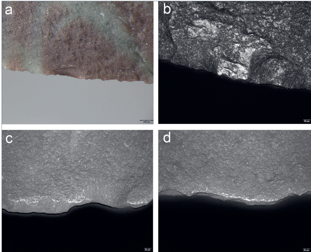
Fig. 7: a) A small bending-initiated scar from working willow on backed piece RM 1 (radiolarite) used for two hours. Original magnification 56×, scale bar 200 µm; b) Polish from working willow on RM 1 (radiolarite) used for two hours. Original magnification 500×, scale bar 20 µm; c) Polish from working willow on RM 4 (Jurassic chert) used for 1.5 hours. The polish is bright and more or less comparable to wood polish on flint in its texture and distribution. Original magnification 500×, scale bar 20µm; d) Polish from working willow on RM 4 (Jurassic chert) used for 1.5 hours. The polish forms a narrow band on the edge and is less characteristic than that shown in 7c. Original magnification 500×, scale bar 20 µm (photos: N. Taipale).
