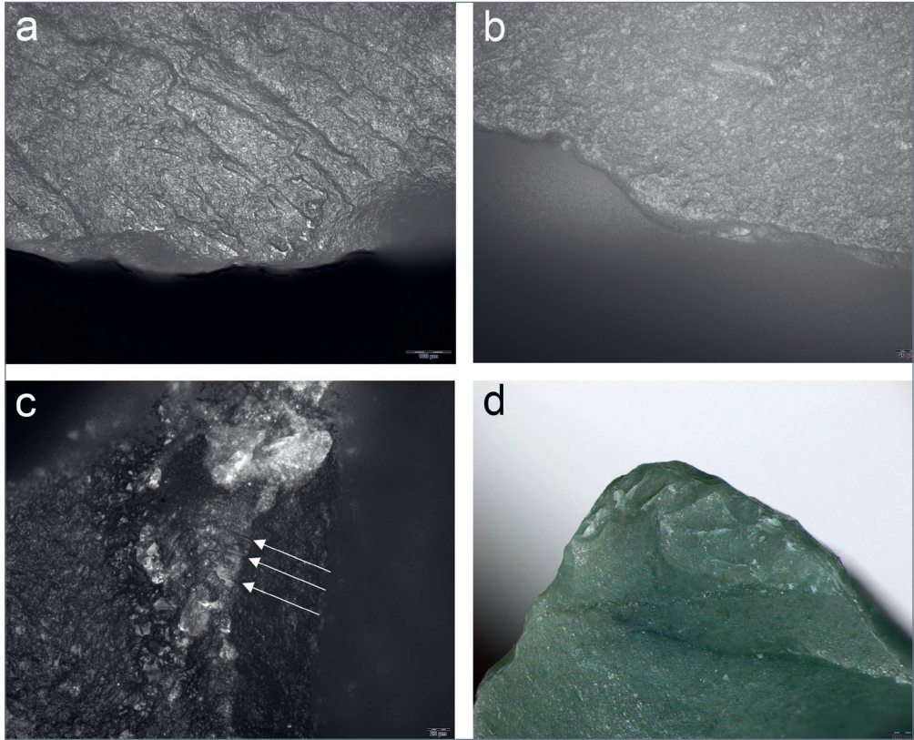
Fig. 11: a) Bright polish on high points of surface microtopography on RM 6 (radiolarite), used for cutting partially tanned rigid hide for 12 minutes. The polish may be influenced by small chips that came off the tool edge and became embedded in the worked material. Original magnification 200 \times , scale bar 100 \mu\text{m} ; b) Edge rounding and polish from perforating partly tanned rigid hide on BO 9 (Jurassic chert), used for 11 minutes. Original magnification 500 \times , scale bar 20 \mu\text{m} ; c) Longitudinally oriented linear polish and striations (indicated with arrows) on the tip of BO 1 (radiolarite), used for perforating a marine shell for 40 minutes. The wear features are caused by either direct contact with the shell or by the chips that came off the tip during work. Original magnification 500 \times , scale bar 20 \mu\text{m} ; d) Crushing (small abruptly terminating scars) on the tip of BO 2 (radiolarite), used for perforating marine shell for ca. 40 minutes. Original magnification 32 \times , scale bar 200 \mu\text{m} (photos: N. Taipale).
