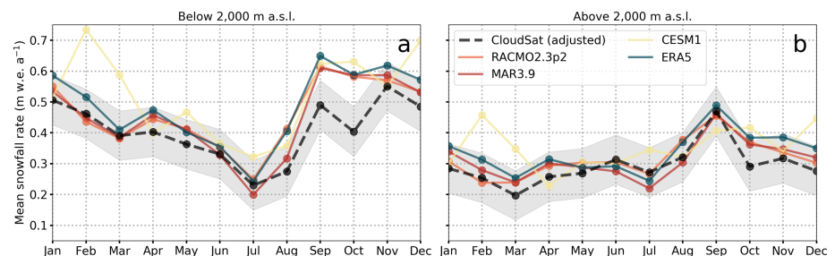
Figure 13. Comparison of CloudSat and modeled monthly snowfall rates averaged over a decade (2006–2016). (a) Monthly snowfall rates below 2,000 m asl. (b) Monthly snowfall rates above 2,000 m asl. The grey shade indicates uncertainty in CloudSat snowfall rates after bias correction ( \pm 0.08 m w.e./a or \pm 17\% ). Generally, the seasonal variation in snowfall is captured by all models in comparison to our bias-corrected CloudSat snowfall climatology. However, below 2,000 m asl, the regional and global climate models appear to overestimate snowfall during autumn.
