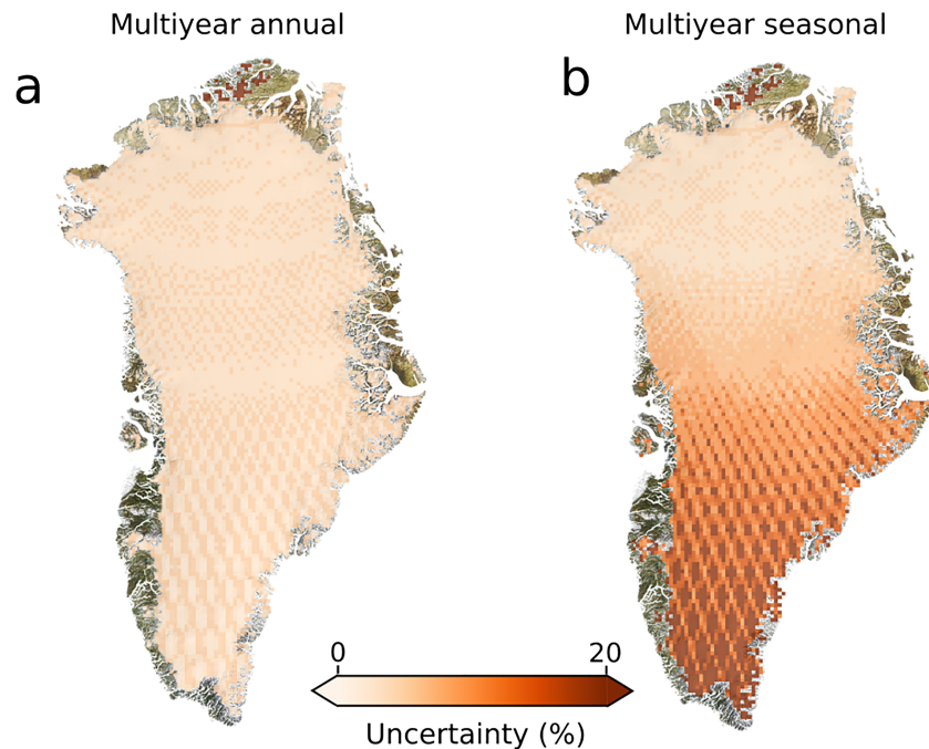
Figure 5. Spatial variability of CloudSat accumulation rate uncertainty due to sampling frequency. (a) The uncertainty due to sampling frequency in the decadal-averaged product is never higher than 5% because all grid cells receive at least 340 observations. (b) The uncertainty for the seasonally averaged product rises to up to 20% in South Greenland because some grid cells only receive 85 observations.
