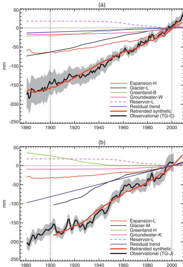
FIG. 10. Two examples comparing an observational and a re-trended synthetic time series of global-mean sea level rise (thick lines, with 5%–95% observational uncertainty shaded), also showing the contributions to the latter (thin lines), identified by the time series initials in the key. In each panel, the observational and the re-trended synthetic time series have the same time mean during 1901–90, and the latter and its components are all plotted relative to zero in 2000. These examples are two of those shown in Fig. 8a; they do not include the adjustment of 0.05 \text{ mm yr}^{-1} applied in Fig. 8b. Panel (b) shows the synthetic time series that gives the smallest RMS difference from the observational time series TG J.
