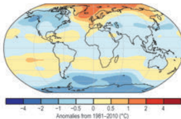
PLATE 2.1. (a) NOAA GlobalTemp surface temperature anomalies; (b) Satellite-derived lake surface water temperature anomalies; (c) GHCNDX warm day threshold exceedance (TX90P); (d) GHCNDX cool night threshold exceedance (TNI0P); (e) ERA5 lower tropospheric temperature grid anomalies; (f) ERA-Interim gridpoint lower stratosphere temperature anomalies; (g) HadISDH annual average anomaly surface specific humidity over land;
