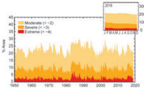
FIG. 2.31. Percentage of global land area (excluding ice sheets and deserts) with scPDSI indicating moderate (<math>scPDSI <-2</math>), severe (<math>scPDSI <-3</math>) and extreme (<math>scPDSI <-4</math>) drought for each month of 1950–2018. Inset: Each month of 2018.
