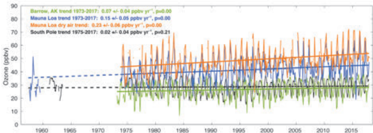
FIG. 2.60. Monthly median ozone at Utqiagvik (Barrow), Alaska (Mar 1973–Dec 2018, green), and South Pole (Jan 1975–Dec 2018, black) using data from all hours of the day. Additional data from South Pole are shown for the early 1960s. Also shown are nighttime monthly median ozone values at Mauna Loa Observatory (MLO) calculated with all available data for months with at least 50% data availability, Oct 1973–Dec 2018 (blue), with early observations from the late 1950s. In addition, the monthly median values associated with dry air masses (orange) at MLO are included (dewpoint < climatological monthly 40th percentile, and a monthly sample size \geq 24 individual hourly nighttime observations). Trends (solid straight lines) are based on least-squares linear regression fit through the monthly values (1970s–2018), and reported with 95% confidence intervals and p -values. The MLO and South Pole trend lines are extrapolated back in time to the late 1950s (dashed lines).
