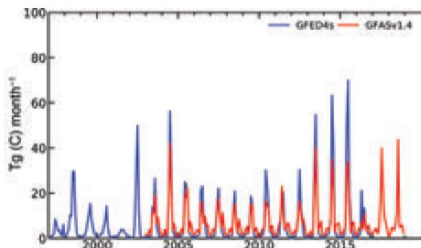
FIG. 2.68. Time series of fire activity during 1997–2018 in terms of carbon consumption [ \text{Tg (C) month}^{-1} ] for North America.
