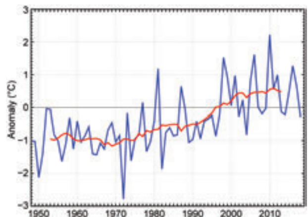
FIG. 7.1. Annual average temperature anomalies (°C; 1981–2010 base period) in Canada for 1948–2018. Red line is the 11-year running mean. (Source: Environment and Climate Change Canada.)
