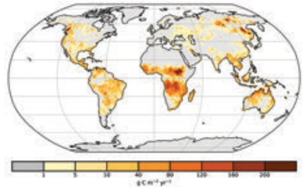
FIG. 2.67. Global map of fire activity in 2018 in terms of carbon consumption ( \text{g C m}^{-2} \text{yr}^{-1} ). (Source: GFASv1.4.)
