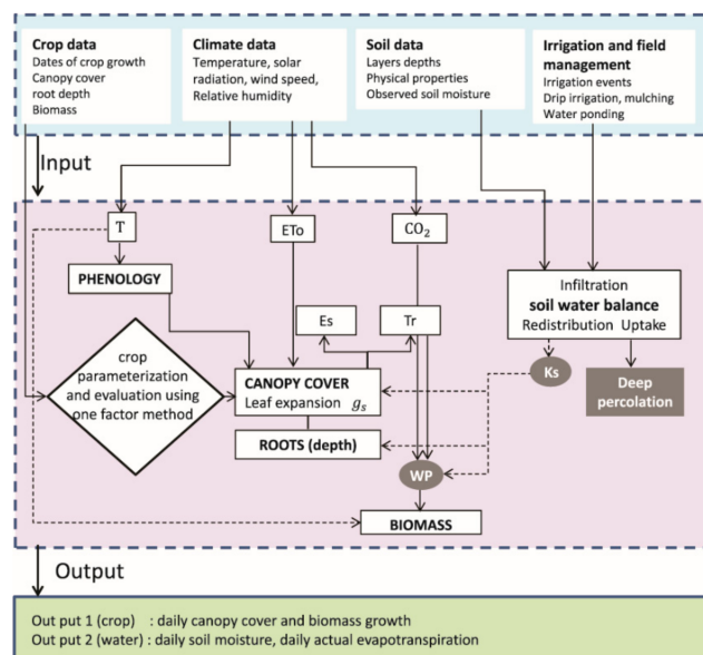
Figure 3. Flow chart of parameterisation of AquaCrop in this study (adjusted from [76]). T is temperature, ETo is potential evapotranspiration, g_s is stomatal conductance, WP is water productivity coefficient, K_s is stress coefficient, E_s is soil temperature, Tr is crop transpiration.
