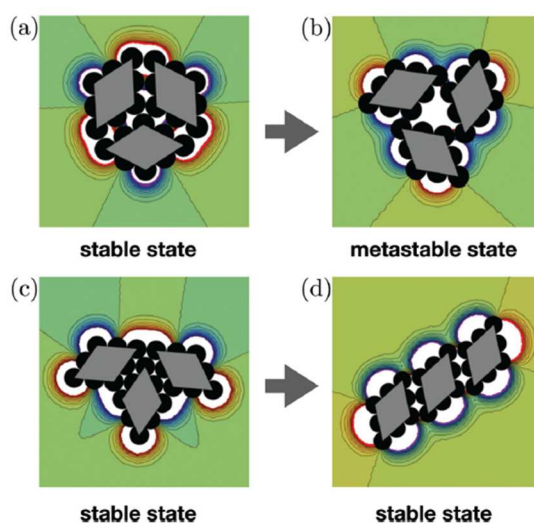
Fig. 8 Two initial different stable rhombic states are driven to a single stable isohedral state when capillary charges are transferred from vertices to sides. For the first compact configuration (a), a metastable state (b) is obtained for which three rhombi form a triangular configurations, as observed in Fig. 1. Another configuration (c) leads to a perfect isohedral stable state (d). The blue-green-red color scale indicates the elevation of the liquid interface in arbitrary units. Blue (red) corresponds to a negative (positive) capillary charge, while the green color corresponds to a flat unperturbed interface.
