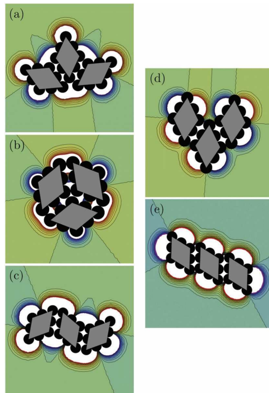
Fig. 4 All resulting patterns made of three objects, resulting from the simulations of capillary attractions and repulsions. The first column (a–c) shows the cases dominated by vertex–vertex interactions starting from different initial conditions. The right column (d and e) shows the cases dominated by edge–edge interactions. The blue-green-red color scale indicates the elevation of the liquid interface in arbitrary units. Blue (red) corresponds to a negative (positive) capillary charge, while the green color corresponds to a flat unperturbed interface.
