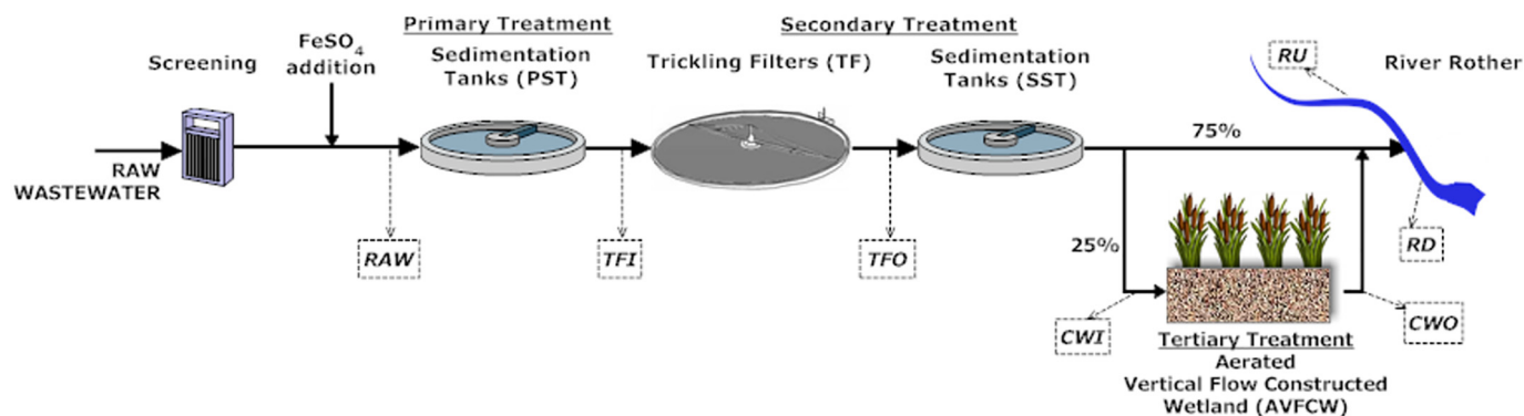
Fig. 1. Schematic representation of the treatment train and sampling points at Petersfield Sewage Treatment Works in South UK (PST; primary sedimentation tanks, TF; trickling filters, SST; secondary sedimentation tanks, AVFCW; aerated vertical flow constructed wetland, RU; river upstream, RD; river downstream).
