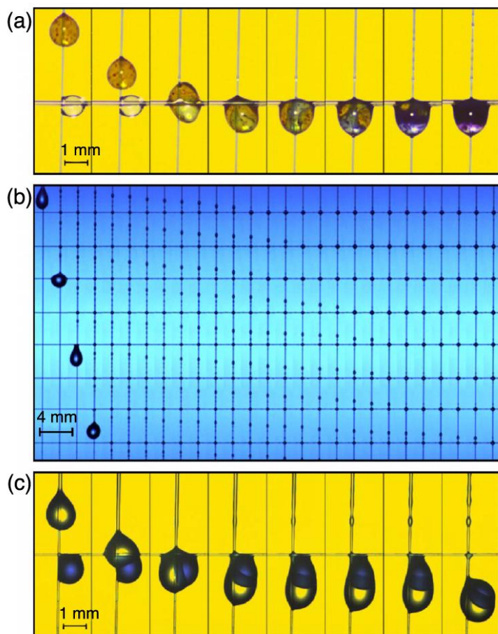
Figure 4. (a) \text{H}_2\text{SO}_4 droplet (upcoming) fuses with a \text{NaOH} droplet on a node. The reaction is revealed by bromomethyl blue. The snapshot length is 0.1 s. (b) With nodes in series, a single large droplet is divided in many tiny droplets. The fluid lost by coating the vertical fiber is collected at junctions. Snapshots are taken every 48 ms. (c) A colored water droplet is placed on a fiber intersection. Then, a 50 cS oil droplet slides down the vertical fiber, wraps the water droplet, and the resulting liquid object leaves the junction. Snapshots are taken every 64 ms (enhanced online). [URL: http://dx.doi.org/10.1063/1.3157141.1 ]
