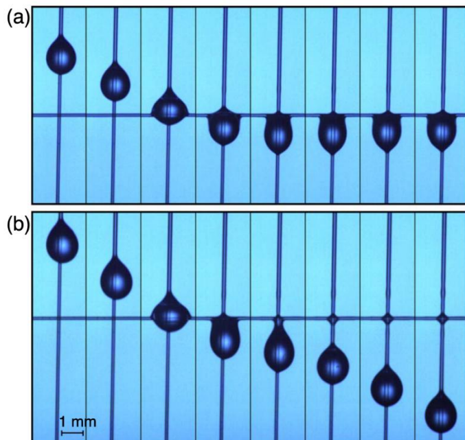
Figure 2. A 5 cS oil droplet interacts with a junction between two nylon fibers (radius 70\mu\text{m} ). Snapshots are taken every 10 ms. The intersection behaves as a fluidic diode: (a) a small droplet is pinned on the junction, while (b) a large droplet crosses it. In that latter case, a tiny amount of liquid is left at the intersection.
