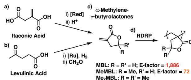
Scheme 9. Transformation of a) itaconic acid [160,162] and b) levulinic acid [161] into c) methylene butyrolactones, and d) the controlled radical polymerization of these monomers into poly( \alpha -methylene- \gamma -butyrolactone)s. [163,164] The reported E-factors exclude column chromatography. [162]
