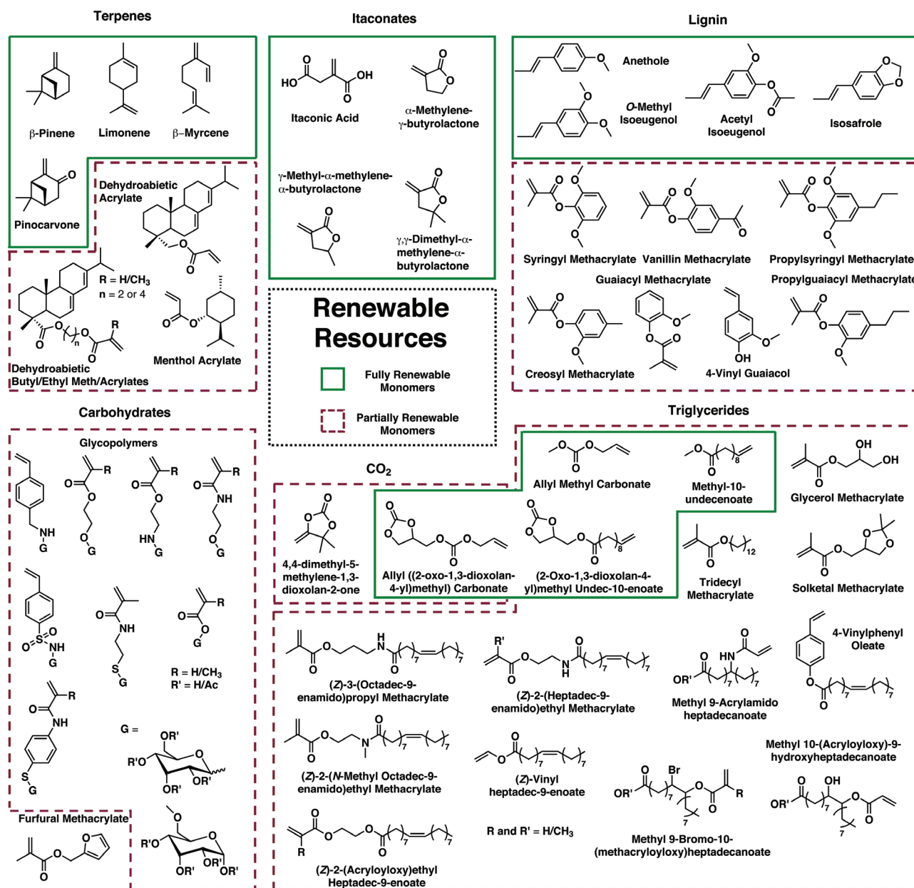
Figure 1. Overview of the types of monomers available from renewable resources that have been polymerized using RDRP techniques. The monomers highlighted by a green square are the subject of this review, while those in a red dashed square are partially renewable and have been summarized elsewhere. [5–8,10–13]
