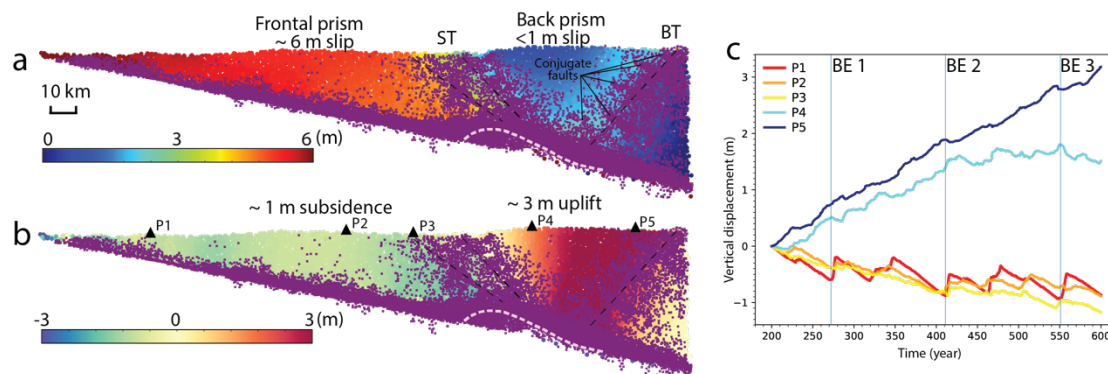
Figure 8: Displacement values of the overriding plate during 400 years (the seamount is represented as a pink dash line) including (a) horizontal component, (b) vertical component; (c) vertical displacement record of points P1-P5 (in (b)) with three vertical light blue lines in order to indicate the positions of the three big events in the model. Cracks (purple dots) align along megathrust faults, splay thrust fault (ST), and back thrust fault (BT), respectively. The color fields reveal that the displacement distribution of the overriding plate. The locations of conjugation faults are identified in (a).
