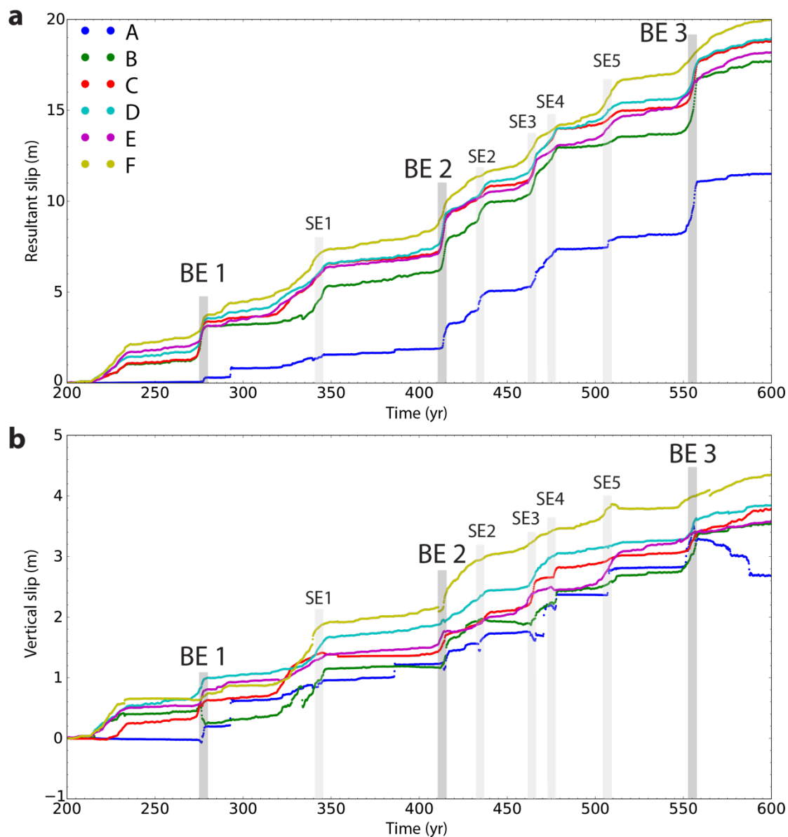
805 Figure 13: The accumulated slip of Point A to F in the frontal prism defined in Figs. 10 and 11: (a) resultant slip and (b) vertical component along the slab. During the big events BE 1-3, the slip suddenly increases, suggesting significant coseismic slips. The accumulative slip from Point A to F increases whereas the coseismic slips of the big events decreases. Between BE1 and BE2, there is a sub-event, SE1. Between BE2 and BE3, there are four sub-events, SE2-5, which can be identified in (a), but are not clear in (b). The key reference locations (Point A to F) are denoted in Fig. 6.
