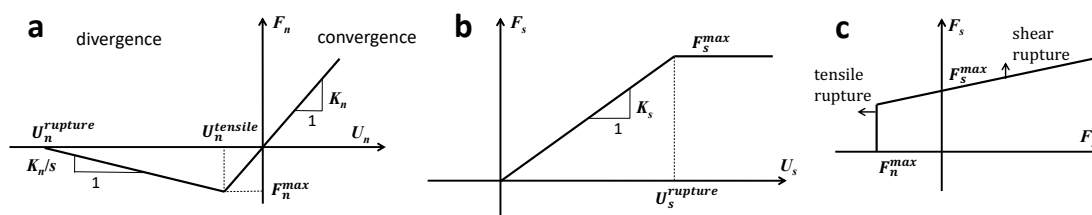
700 Figure 2: The contact model used in the simulations: (a) normal behavior, (b) tangential behavior, and (c) failure envelope.
