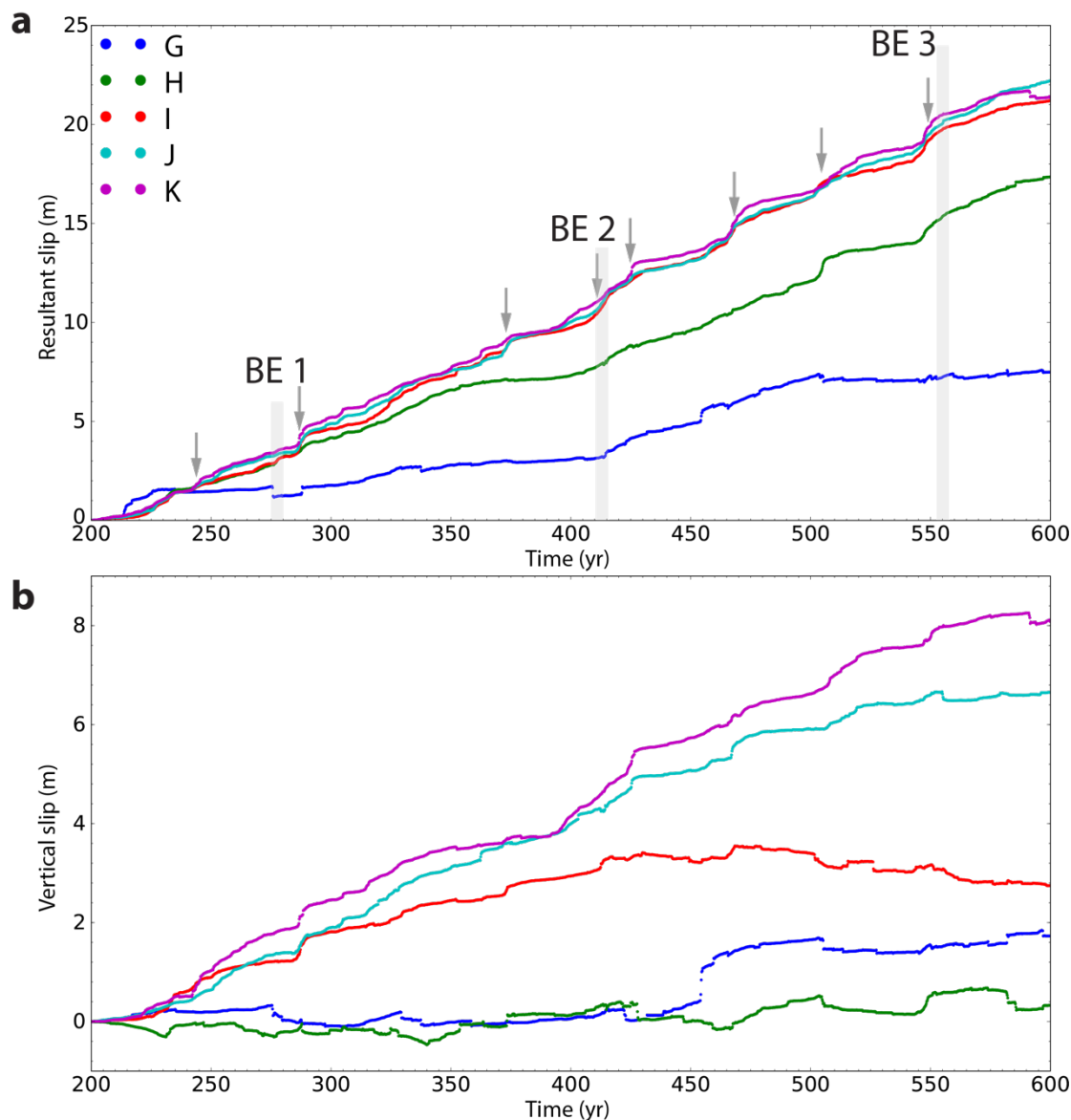
810 Figure 14: The accumulated slip of Point G to K which are close to the seamount as denoted in Figs. 10 and 11: (a) resultant slip and 815 (b) vertical component along the slab. Gray arrows, which are different from the light gray bars (BE1-3), indicate the small co-rupture slips during smaller events from Point I to K curves. Point G and H are close to the seamount, thus co-rupture slip behaviors around them are more complex. The slips generally increase from Point G to K. Their slip patterns show more co-rupture slips of frequent small events, which are related to the events slip along the splay fault. The vertical component pattern shows the local seamount geometry effect. The key reference locations (Point G to K) are denoted in Fig. 6.
