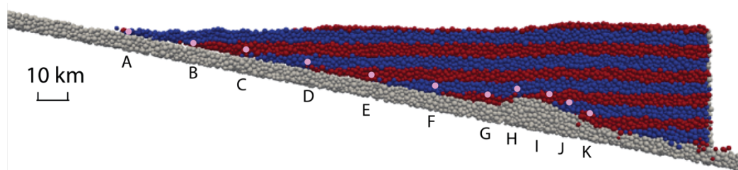
Figure 6: The initial state (initial balance situation): the layers with different colors inside the overriding plate help identify how the overriding plate deformed; the key reference locations (Point A to B just above the slab and Point C to K ca. 5 km above the slab) are marked here for the later analysis.
