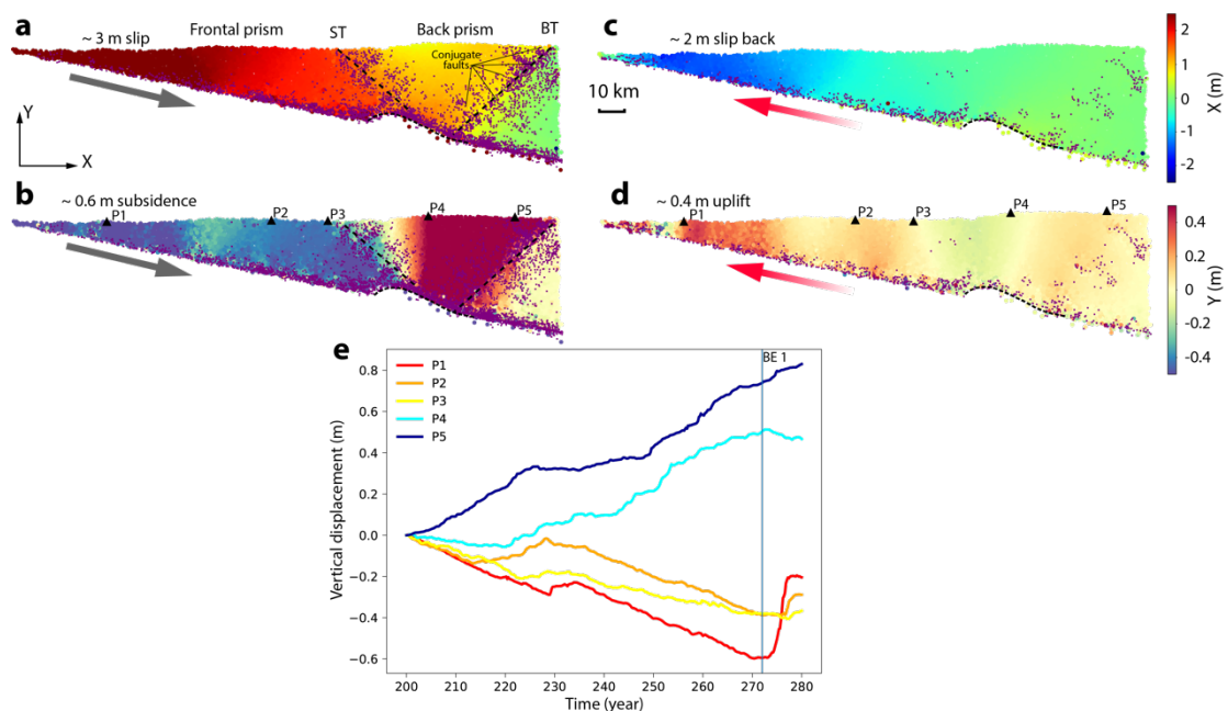
Figure 9: Displacement values of the overriding plate during the first cycle (80 years), which is identified from Fig. 8c: (a) and (b) are horizontal and vertical components respectively before the first big event, (c) and (d) are horizontal and vertical components respectively during the first big event, (e) records the historical path of Points 1-5 in the first cycle and the vertical light blue line is the start position of the first big event; Cracks, ST, BT, P1-P5 and conjugate faults are the same as Fig. 8. Grey and red arrows show the movement direction of the overriding plates before and after the big event respectively.
