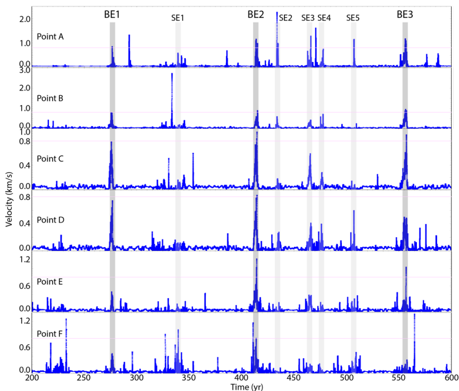
Figure 15: Instantaneous velocity spectrums of Point A to F in the frontal prism along the slab during the simulated 400 years. Three main peaks can be identified corresponding to the big events BE1-3. There are also smaller peaks related to sub events SE1-5. The amplitude of the three main peaks decreases from Point A to F. Note that the velocity at each Point does not use the same scale. The horizontal light pink line corresponds to a velocity of 0.8 km/s, for reference. The key reference locations (Point A to F) are denoted
