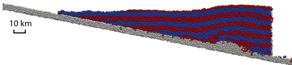
Figure 7: Final deformation after ca. 400 years.
