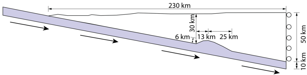
Figure 4: The model geometry: the right boundary of the overriding plate is fixed, and the slab is subducting at ca. 6.12 cm/year.
