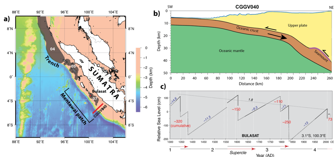
685 Figure 1: (a) Geological setting at the Mentawai zone. The location of the CCGV040 seismic reflection profile (red line) and the location of the paleoseismic history study (red dot) are located on the Mentawai patch. The three grey semi-transparent areas from north to south are ruptures of M9.2 (2004), M8.6 (2005) and M8.4 (2007), respectively; b) the interpreted cross-section of the CCGV040 (Singh et al., 2011) shows the geometry of the subducting slab with a seamount (in a purple shape) at the depth of ca. 30- 40 km; c) earthquake cycles from the paleoseismic records at Bulasat (Sieh et al., 2008) show the big rupture events repeat every ca. 200 years and result the vertical slips of ca. 0.7 – 2.5 m. In addition, this paleoseismic model infers that the big rupture event at the 690 Mentawai zone will repeat in the future.
