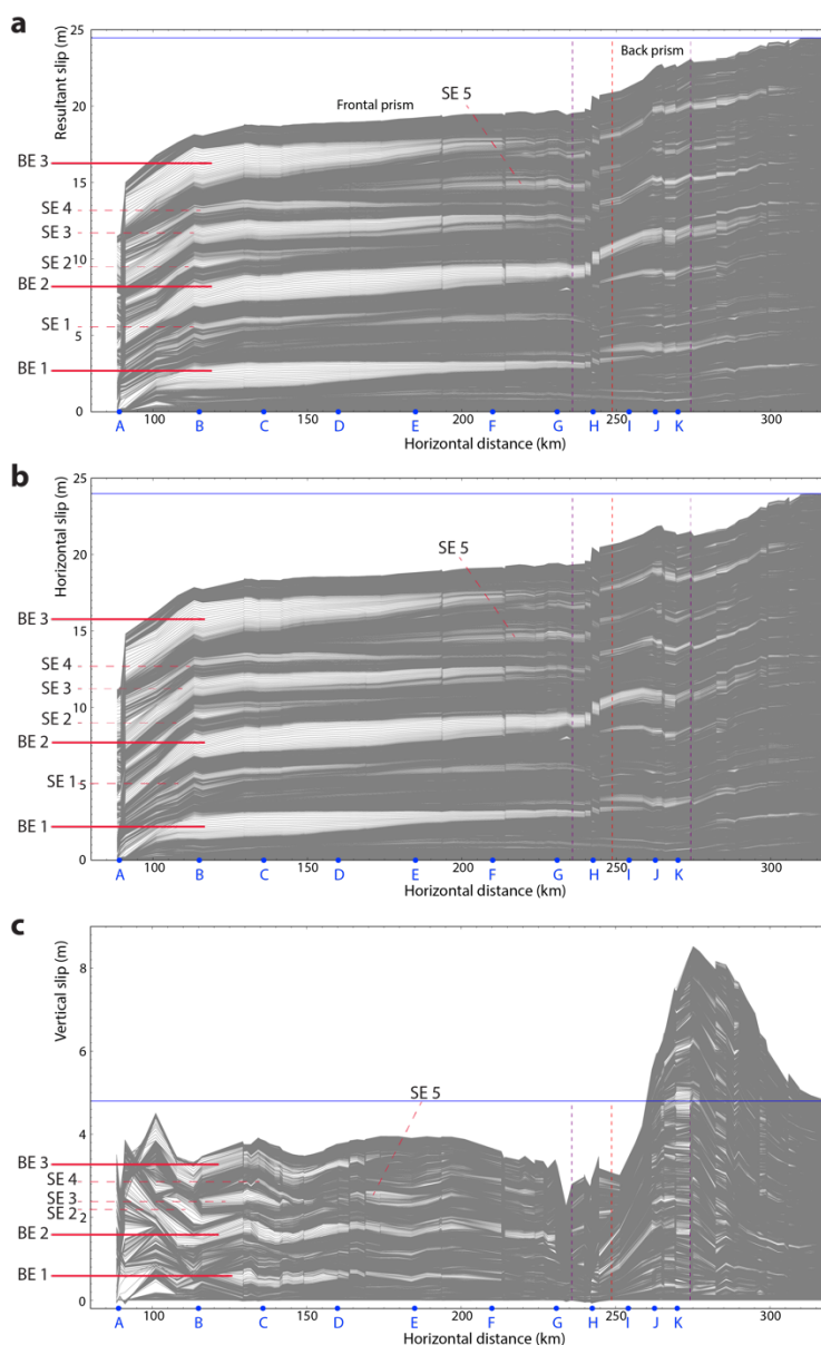
Figure 10: Accumulated slip along the slab interface measured during the simulated 400 years of subduction: (a) accumulated resultant slip relative to the slab, (b) horizontal component and (c) vertical component. Gray lines show accumulated amount of slip along the slab every 0.2 years. The lighter areas reflect fast slip associated with big events. These big events (BE1-BE3) rupture ca. 100 km of the slab interface. Sub-events (SE1-SE5) only rupture smaller patches (ca. 50 km). At the front of the accretionary prism, slip events mostly rupture the slab interface. In the back of the prism, most events produce uplift deformation, with relatively shorter rupture length. The left purple, red and right purple dashed lines show the sites of the seaward base, summit and landward base of the seamount, respectively. The left purple and red lines bound the splay fault nucleation region along the slab. The key reference locations (Point A to K) are denoted in Fig. 6.
