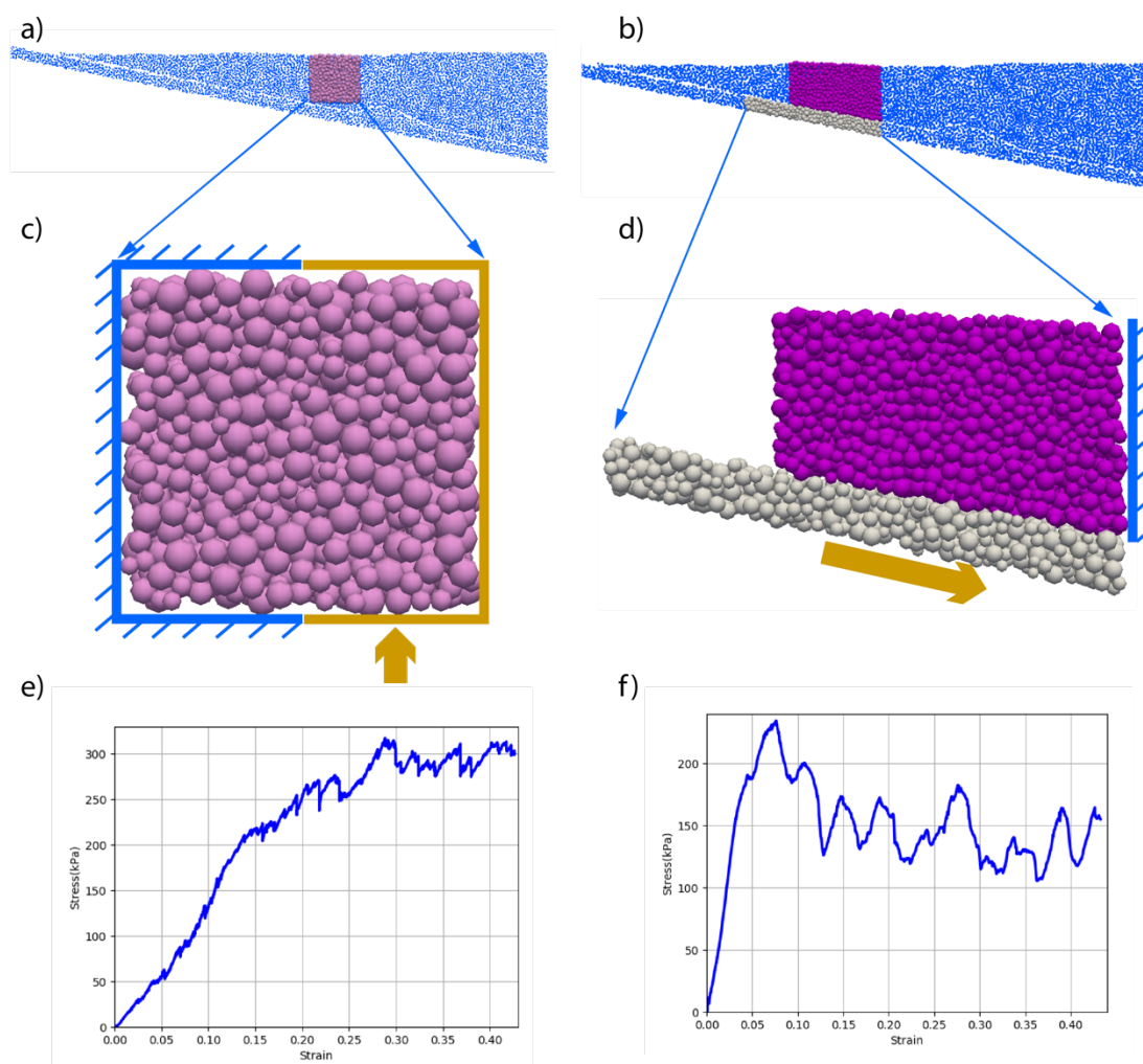
Figure 5: Modeling calibration includes two shear tests for the generated and pre-existing fault. (a) and (b) show the blocks we took from the entire model for the shear tests. (c) shows the simple shear test setting for the generated fault: the blue boundaries are fixed, and the shear loading is exerted on the yellow boundaries. Since we simulate the fault strength on average at depth \sim 15 km, we also apply the \sim 400 kPa (hydrostatic pressure \rho gh ) lateral stress in this test. (d) shows the shear test for the pre-existing fault, which is part of the simulated megathrust fault: the blue boundary constrains the displacement of the purple block, and the loading velocity is applied on the white block. (e) and (f) show the stress-strain curves of the generated fault and pre-existing faults respectively.
