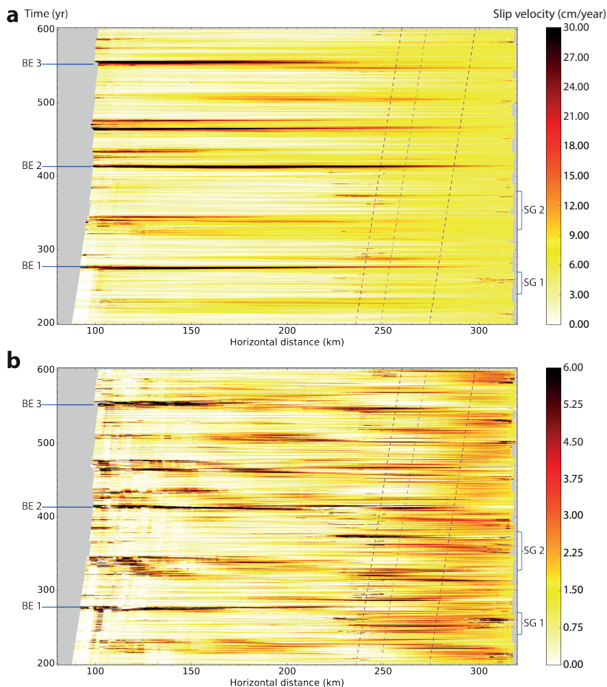
795 Figure 12: Slip velocity spectrum along the top surface of the overriding plate: (a) resultant slip velocity; (b) vertical component of the slip velocity. Surface slip amount also show the big events and sub-events; but the light yellow region (between the left purple and gray dashed lines) is not as clear as that in Fig. 11; the splay fault group rupture longer over the entire seamount, because of the dip of the splay fault (Figs. 8 and 9). The left purple, gray and right purple dashed lines are the sites of the seaward base, summit and landward base of the seamount, respectively.
