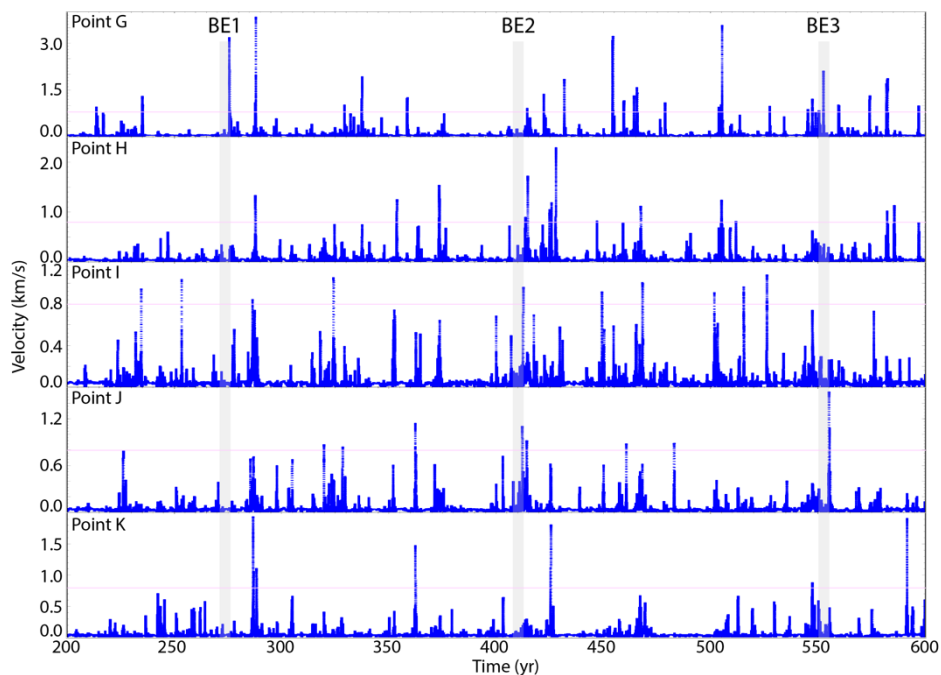
835 Figure 16: Instantaneous velocity spectrums of Point G to K close to the seamount along the slab during the modeled 400 years. Many small events can be identified. The big events BE1-3 (indicated by light gray bars) do not cause significant peaks in these spectrums. The horizontal light pink line corresponds to a velocity of 0.8 km/s, for reference. The key reference locations (Point G to K) are denoted in Fig. 6.
