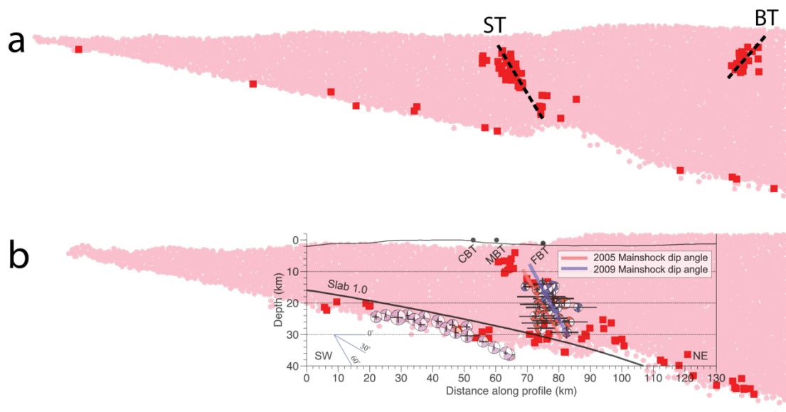
Figure 18: Crack swarms at (a) the beginning and (b) the end of the simulation period. The crack swarms are compared to the seismic observations in (Wang et al., 2018) . The locations and the dip angles of the slab and the splay fault (ST) are consistent with observations.
