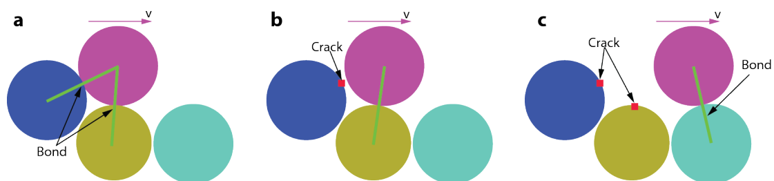
710 Figure 3: Illustration of kinematics and interparticle bond behavior for particles initially in contact (a) and generation of cracks (b) and the new bond (c). The purple particle is moving towards the right side.
