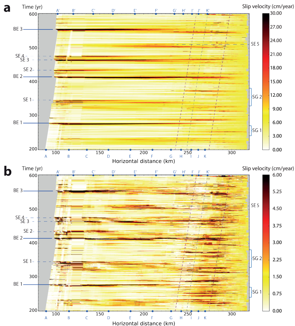
790 Figure 11: Slip velocity spectrum along the slab: (a) resultant slip velocity and (b) vertical component of slip velocity along the slab. The recurrence interval of big events is ca. 140 years. Relatively smaller events concentrated along the splay fault (e.g. events in SG1-2) are best observed in the vertical component distribution. Every line represents the slip velocity along the slab per scaled 0.2 years over the simulated 400 years. The left purple, gray and right purple dashed lines are the sites of the seaward base, summit and landward base of the seamount, respectively; light yellow region on the seaward side of the seamount indicates lower slip rate along the interface; The key reference locations (Point A to K) are denoted in Fig. 6.
