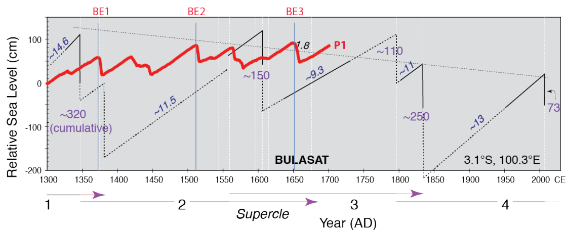
845 Figure 17: Comparison of the vertical motion of the point P1 in the modeling and paleoseismic observations made in Bulasat in the Mentawai area from Sieh et al. (2008). See more details in Fig. 1 and 8 above.
