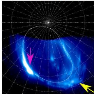
Figure 1. Auroral examples with synchronized auroral dawn storm (pink arrows) and auroral injection (yellow arrows).
