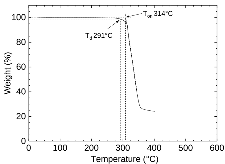
Figure S1: Example of T_d and T_{on} graphical determination on a Pyr 13 FSI thermogram.
