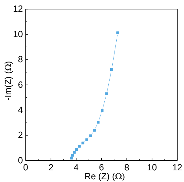
Figure S2: Example of an electrochemical impedance spectrum of a \text{LiCoO}_2/\text{GPE}/\text{Cu} configuration ("Li-free") at open circuit voltage just after the assembly.
