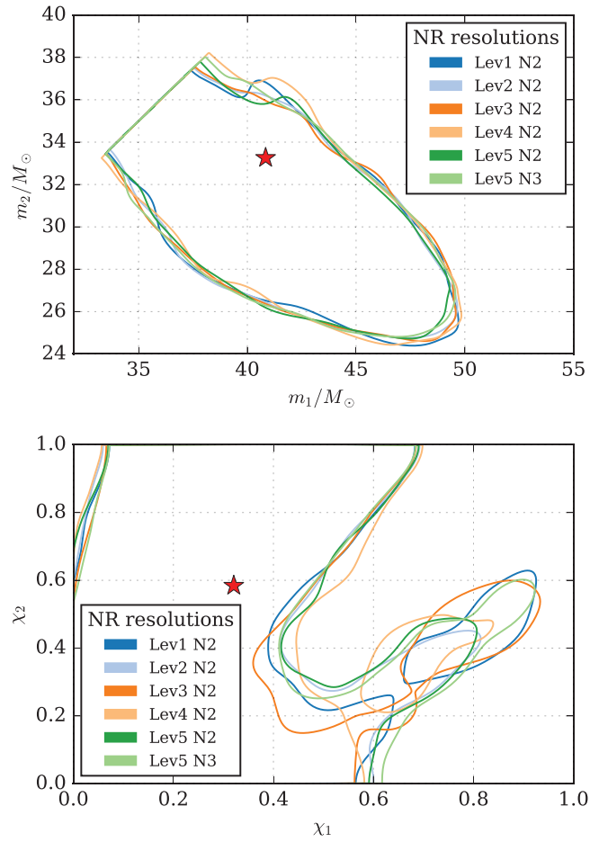
Figure 9. 90% credible regions for configuration SXS:BBH:0308 with numerical resolutions Lev = {1, 2, 3, 4, 5} and extrapolation orders N = \{2, 3\} . We find consistent results between the different resolutions and extrapolation orders, indicating that numerical errors are a negligible source of parameter biases.
