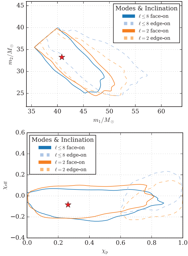
Figure 6. Results for processing NR injections (SXS : BBH : 0308) with face-on or edge-on inclination ( \theta_{\text{JN}} = 6^\circ and 84^\circ , respectively) and either including higher harmonics up to \ell = 8 (compare with figure 4) or just the \ell = 2 modes in the mock signal. All injections are performed at fiducial polarization angle \psi = 82^\circ . The precessing IMRPhenom model is used as the template waveform. We show two-dimensional 90% credible regions for component masses and effective spins.
