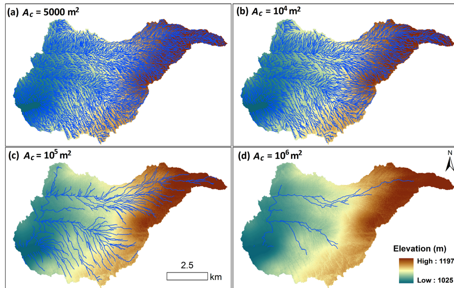
Figure 6. Variable supraglacial stream and river network for IDC1, as simulated by applying variable accumulative area threshold (channel initiation threshold, A_c ) values to ArcticDEM.
