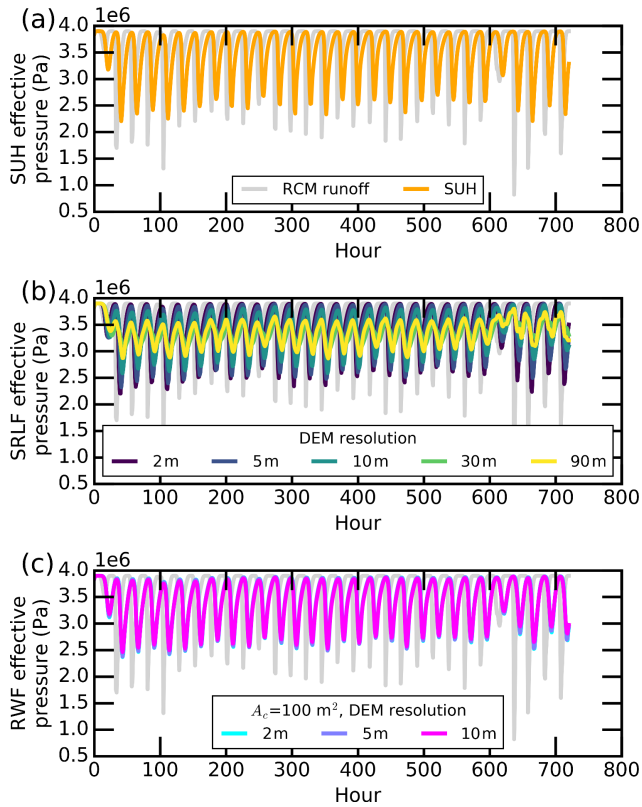
Figure 3. Subglacial effective pressures for IDC1 as simulated by SHAKTI, with inputs to the subglacial system via a single moulin prescribed by the moulin discharges (shown in Fig. 2) generated by the various surface meltwater routing models. The effective pressure shown is the spatial mean over the entire 1 km square domain, which contains the moulin input at its center.
