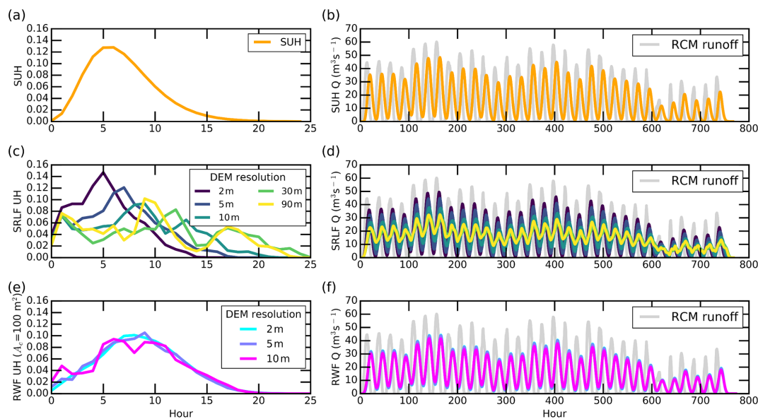
Figure 2. Presentation of unit hydrographs (UHs; column 1) and moulin discharges (column 2) of IDC1 during July 2015, as simulated by three surface meltwater routing models (SUH, RWF, and SRLF). Simultaneous RCM runoff (gray line) is shown to indicate the effect of surface meltwater routing processes on moulin discharge.
