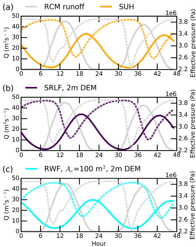
Figure 5. The average 2 d cycle of moulin discharge ( Q ) for IDC1 during July 2015 derived from Figs. 2 and 3. The daily minimum input in supraglacial moulin discharge (solid lines) corresponds generally to maximum effective pressure (dashed lines) and is followed within 8–9 h by the daily minimum effective pressure (maximum subglacial water pressure). This suggests that the system shuts down due to creep with low meltwater input and becomes highly pressurized as meltwater input increases again. As the new water inputs are accommodated, efficient pathways reform, and effective pressure increases (subglacial water pressure decreases).
