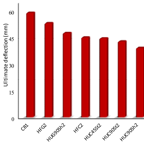
Fig. 10 - Effects of retrofit schemes on ultimate deflection.
