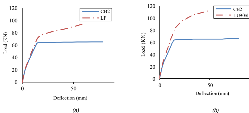
Fig. 8 - Load-deflection curve for beams with 14.2% rebar corrosion: (a) retrofit method 1 (LF) (b) retrofit method 2 (LU90Sh).
