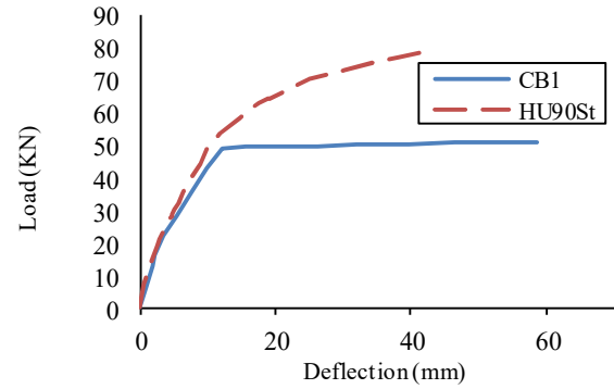
Fig. 6 - Load-deflection curve for beam HU90St.
