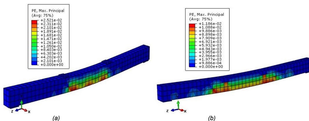
Fig. 13 - The distribution of plain strain for: (a) Strengthen method1 (HF) (b) Strengthen method2 (HU90Sh).
