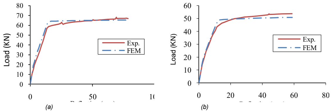
Fig. 2. Comparison of load- deflection relations from experiment and FEA: (a) CN-110 (b) CN-310.
