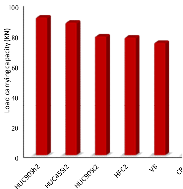
Fig. 9 - Effects of retrofit schemes on load carrying capacity.
