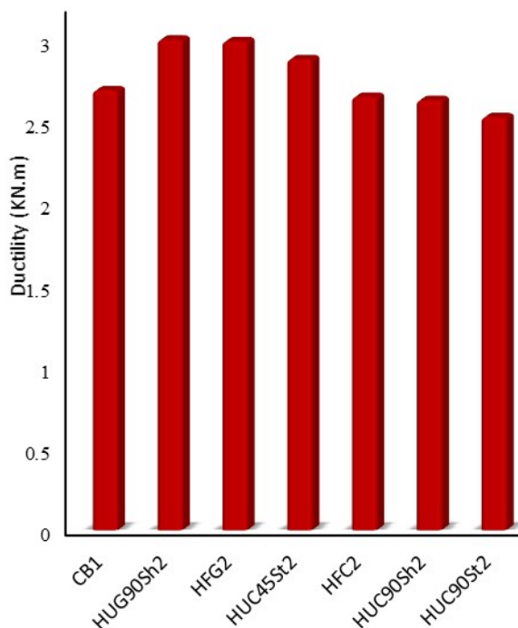
Fig. 11 - Effects of retrofit schemes on ductility.
