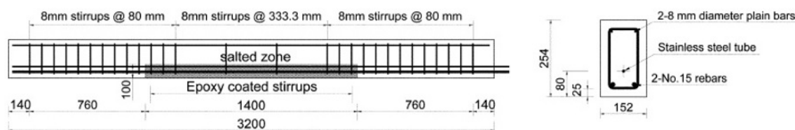
Fig. 1 - Details of test specimens [10].
