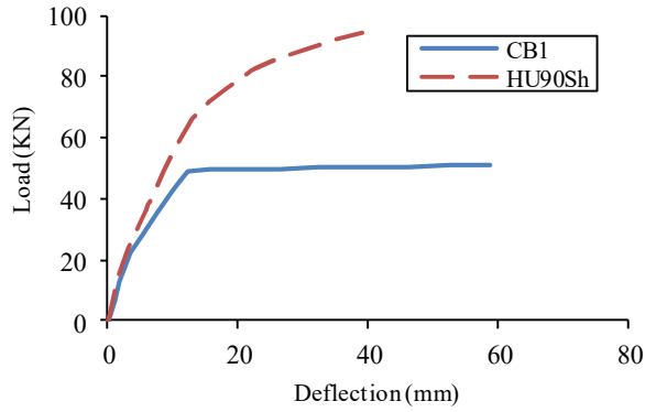
Fig. 5 - Load-deflection curves for beam HU90Sh.
