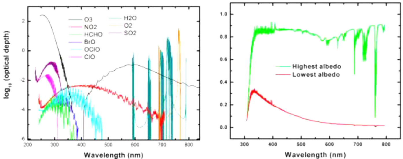
Fig. 4. Left: Absorptions due to molecules that are now commonly measured from space in the nadir geometry; Right: Back scattered albedo spectra from GOME measurements for two extreme examples. The highest albedo scene, corresponding to full coverage by high clouds, is white and quite bright, due to the cloud reflectance; the lowest albedo case is a cloud-free scene over the ocean [30].
