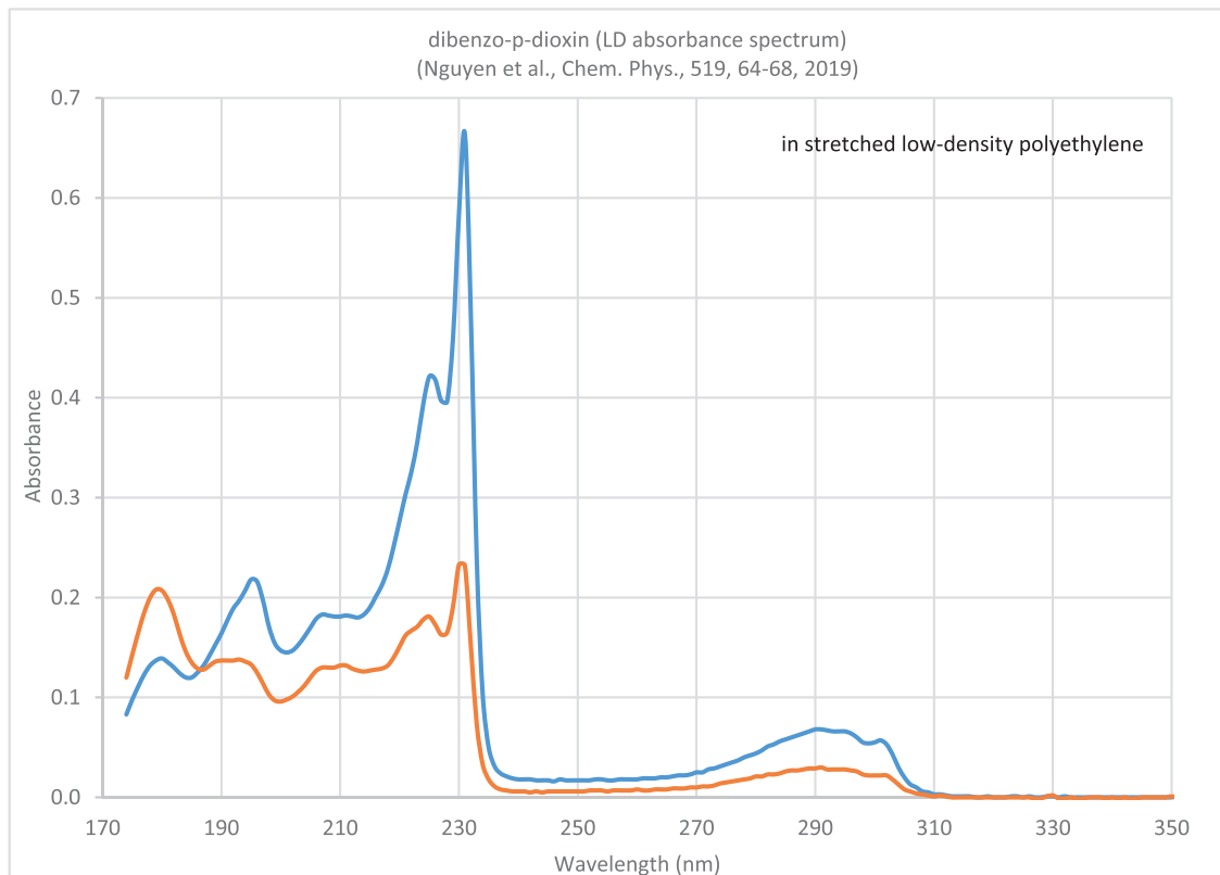
Fig. 2. Linear dichroism absorbance spectrum of dibenzo-p-dioxin [12]. The absorbance curves were recorded with the electric vector of the sample beam parallel (blue line) and perpendicular (orange) to the stretching direction of the polyethylene polymer.
