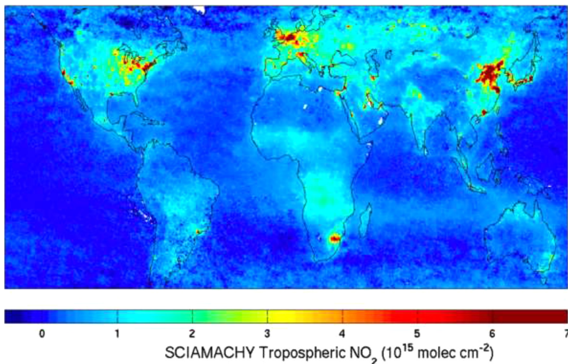
Fig. 5. Tropospheric \text{NO}_2 retrieved from SCIAMACHY measurements in the 425–450 nm spectral region. Pollution on urban scales is readily measured globally [30].
