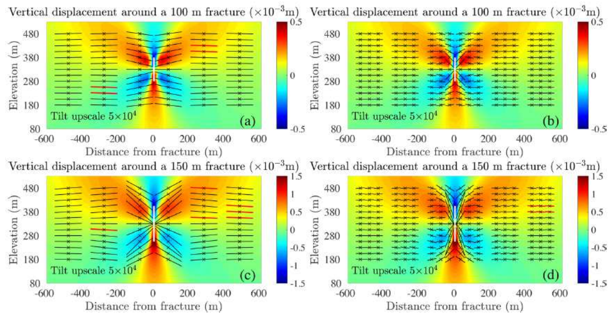
Figure 9. Vertical displacement and induced tilt around a fully loaded fracture, represented by the white vertical line. The initial state corresponds here to an empty fracture. Example with a 100 and a 150 m height fracture (a, b and c, d respectively). Tilts are illustrated for 150 and 50 m length baselines (a, c and b, d respectively). Panels (b) and (d) allow then checking the tilt gradient. Red lines highlight tiltmeters location in agreement with measured tilt amplitude variation (a and c) or a correct tilt amplitude variation and tilt gradient from a small baseline to another (b and d).
