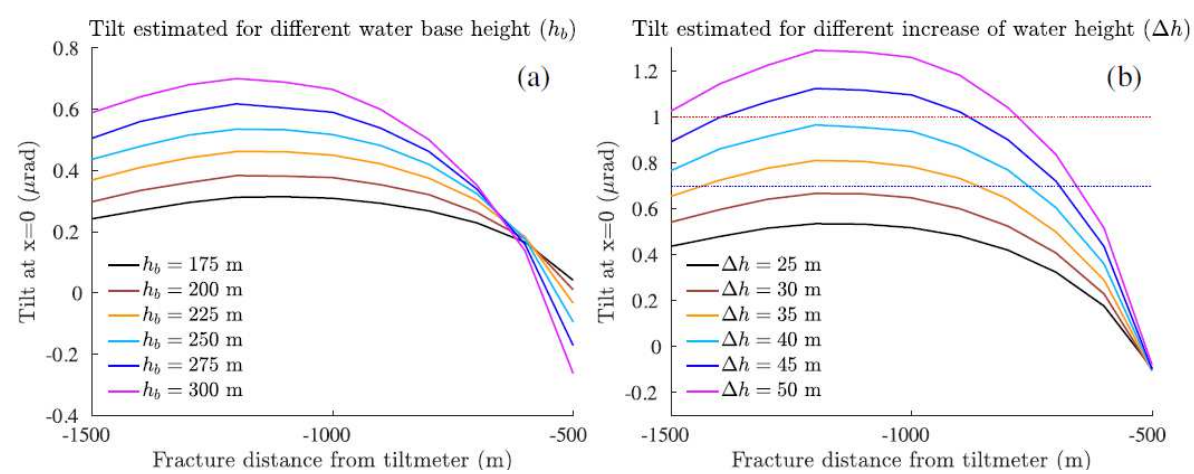
Figure 11. (a) Tilt estimated for different water base heights ( h_b ) following a water level increase of \Delta h = 25 m in a 350 m fracture. (b) Tilt estimated for different water level increase \Delta h for a 350 m fracture and a water base level of h_b = 250 m.
