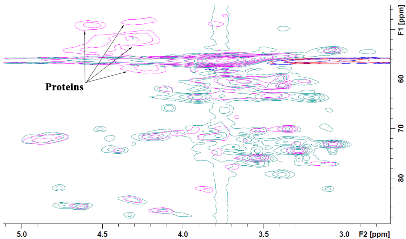
Figure S2: Overlaying of lignin 2D HSQC NMR spectra of E (pink) and E' (green) that highlight the presence of some proteins in the lignin recovered after the first thermic treatment only according to the chemical shift area proposed by Liitia et al., 2003
