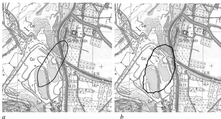
Figure 3: Comparison of odour plume at 1 ou/m 3 for 100 000 ou/s emission rate, wind from 210°, speed 4.7 m/s, Hallembaye site a. Gaussian 2D model – b. Eulerian 3D model.
