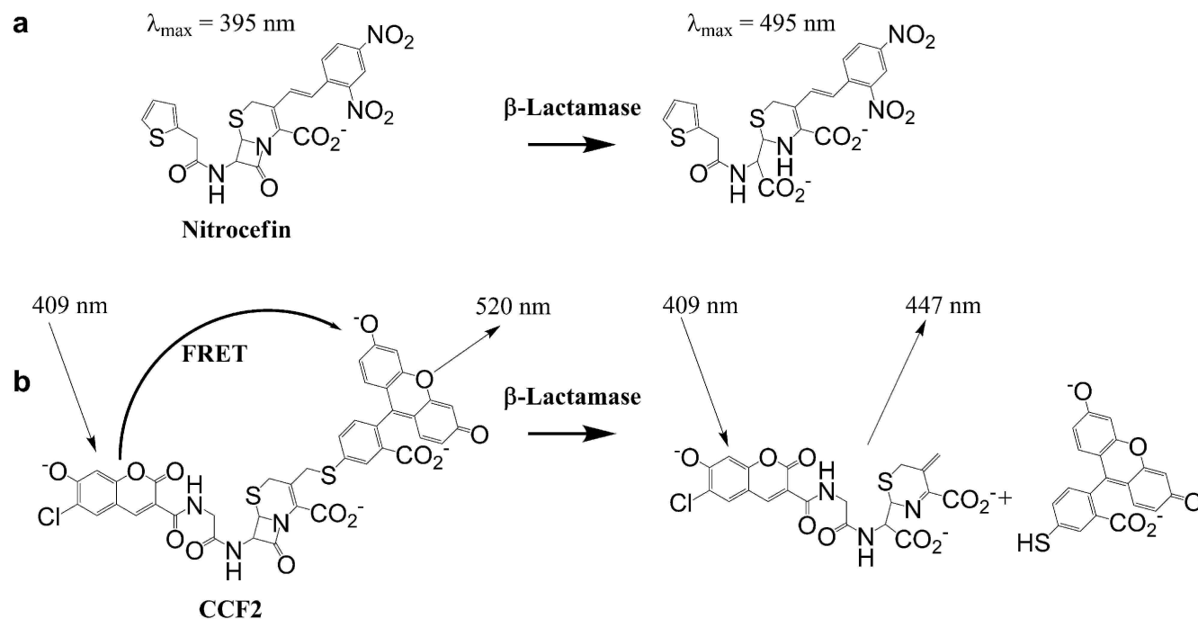
Figure 1. (a) Nitrocefirin assay principle. A change in absorbance at \lambda = 495 nm is measured after the cephalosporin core of nitrocefirin is hydrolyzed by \beta -lactamase, (b) CCF2 (FRET) assay principle. In the intact CCF2 substrate, coumarin moiety's donor FRET resulting from \lambda = 409 nm excitation is efficiently quenched by the acceptor fluorescein moiety; hydrolysis of the \beta -lactam leads to the increase of a donor fluorescence measured at 447 nm and simultaneous decrease of an acceptor fluorescence at measured at 520 nm.
