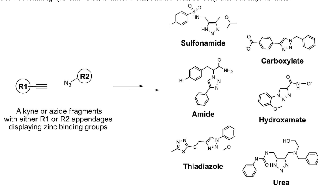
Figure 4. Click-chemistry strategy to synthesize selective VIM-2 inhibitors. Representative N -substituted and N -unsubstituted 1,2,3-triazoles from alkyne and azide fragments with known or putative zinc binding groups are shown including hydroxamates, amides, ureas, thiadiazoles, carboxylate, and sulfonamides.
