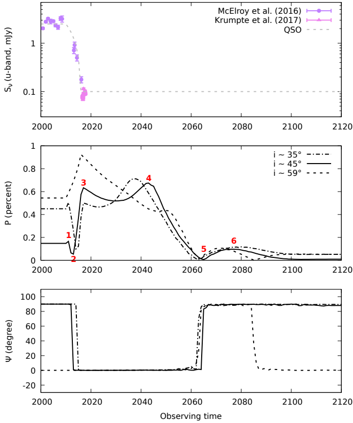
Fig. 6. Top panel: time series of archival u -band flux density S_u for the AGN in Mrk 1018 (McElroy et al. 2016; Krumpe et al. 2017). The host galaxy contribution has been carefully removed by the authors. We plot in gray the flux function we used in our simulation to mimic the dimming of the AGN (host contribution removed). Middle and bottom panels: model predictions for the polarization degree and polarization angle for different nuclear inclinations. See text for an explanation of the red numbers.
