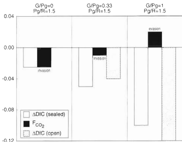
Fig. 1 Numerical example of the effect of organic and inorganic carbon metabolism on seawater inorganic carbon after incubation in a closed volume ('sealed') and upon opening of the incubation chamber to the atmosphere ('open'). P_g : gross primary production; R : respiration, G : net calcification
