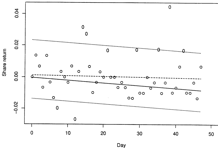
Fig. 1. Share relative returns and fitted models against time: 0, outlying observed returns; ○, observed returns; —, fitted mode under the stable model (d); ·····, 10% relative density contours under the stable model (d); - - - -, mean under the normal model (l)
