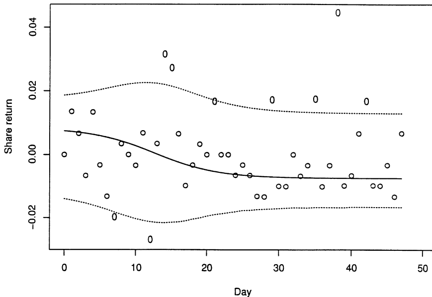
Fig. 3. Share relative returns and fitted stable model (i) against time: 0, outlying observed returns; \circ , observed returns; —, fitted mode; ·····, 10% relative density contours
