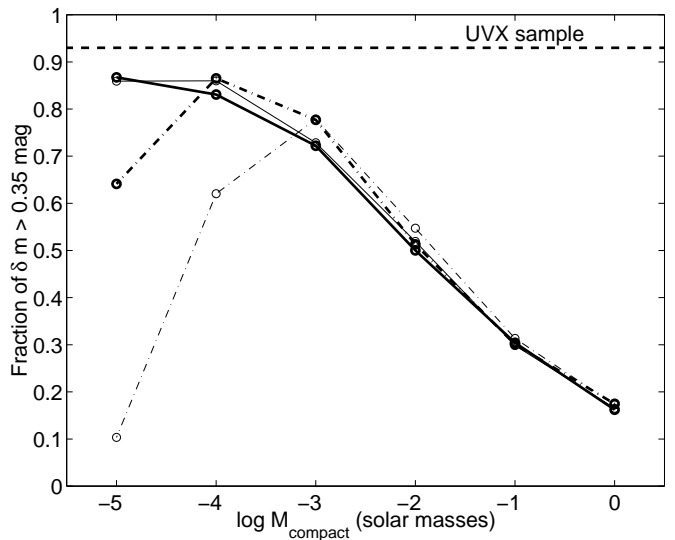
Fig. 5. The fraction of objects with amplitudes higher than 0.35 magnitudes predicted by microlensing scenarios for different M_{\text{compact}} , assuming \Omega_{\text{compact}} = 0.3 , \sigma_{\text{v,compact}} = 600 km/s and R_{\text{QSO}} = 10^{12} m (thick solid), 3 \times 10^{12} m (thin solid), 10^{13} m (thick dash-dotted), 3 \times 10^{13} m (thin dash-dotted). The thick dashed line marks the observed fraction (93%) of the UVX quasar sample.
