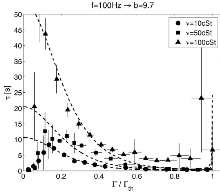
FIG. 3. Lifetime \tau of bouncing droplets as a function of the normalized acceleration \Gamma/\Gamma_{th} for various droplet viscosities. (●) \nu = 10 cSt, (■) \nu = 50 cSt, and (▲) \nu = 100 cSt. Solutions of the model are represented by dashed curves. The frequency ( f = 100 Hz) corresponds to a value of b equal to 9.7.
