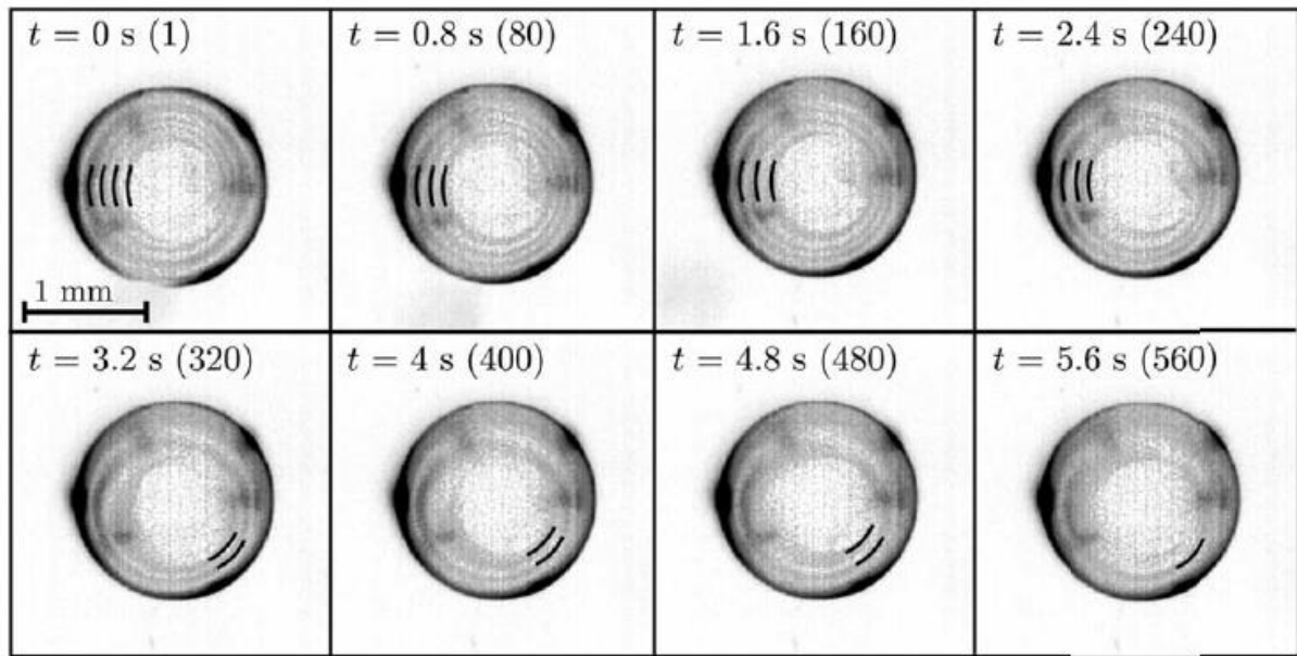
FIG. 5. Successive snapshots of the interference fringes (accentuated by black arcs) taken when the air film thickness is minimal for a droplet bouncing at f = 100 \text{ Hz} , \Gamma = 0.22 \Gamma_{th} , and \nu = 100 \text{ cSt} . The number of fringes decreases with time, indicating a progressive decrease in the average film thickness. The number of bounce from the start is indicated in brackets on each snapshot.
