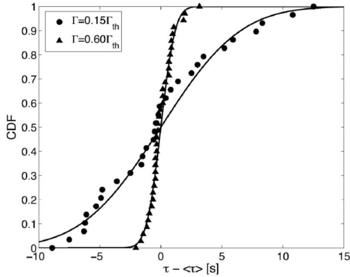
FIG. 2. Cumulative distribution F of the normalized lifetime of bouncing droplets ( f = 75 Hz, \nu = 10 cSt) at various forcing accelerations: (i) \Gamma/\Gamma_{th} = 0.15 (●) and (ii) \Gamma/\Gamma_{th} = 0.6 (▲). The lines represent fitted Gaussian distributions.
