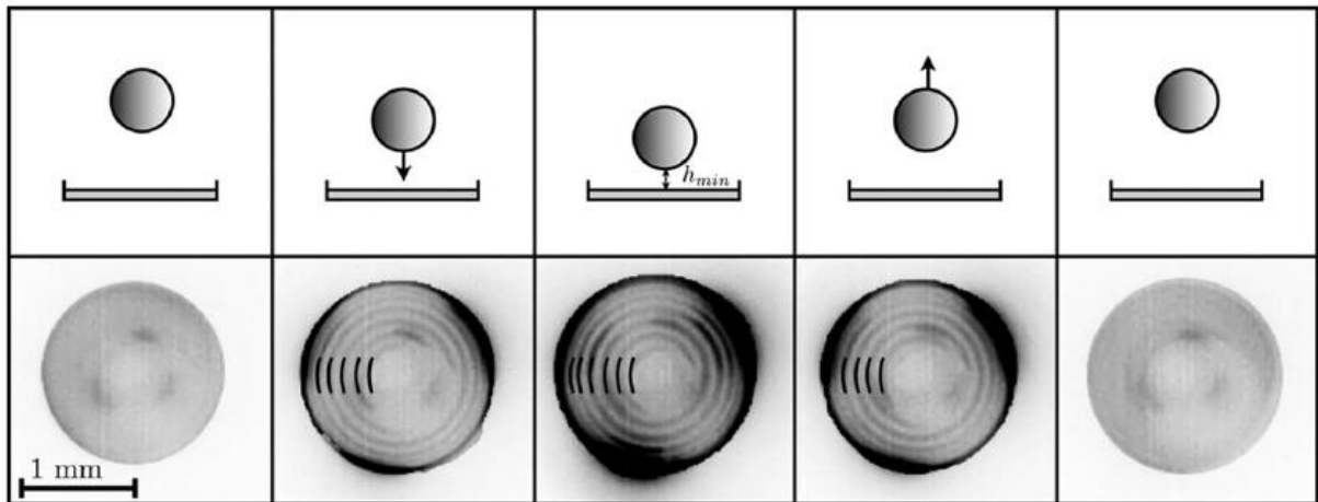
FIG. 1. Successive snapshots of interference fringes (accentuated by black arcs) made by a bouncing droplet. The snapshots are separated by 8 ms. The number of observed fringes is directly related to the film thickness which oscillates in between 100 nm and 10 \mu m. An increasing number of fringes are visible when the droplet lands and squeezes the air film (until snapshot 3); then this number decreases as the droplet takes off.
