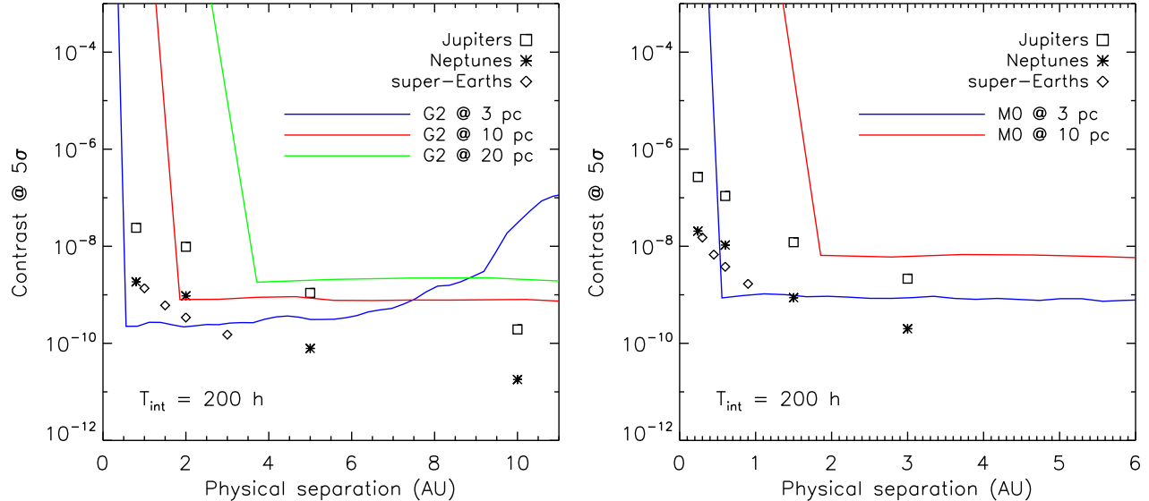
Figure 4. Mean radial profiles of the 5\text{-}\sigma detection level for a G2-type star (left) and a M-type star (right). The curves are plotted for several star distances assuming photon noise and a total integration of 200 h. The planet/star contrast and star-planet separation are derived from Eqs. 2 and 3.
