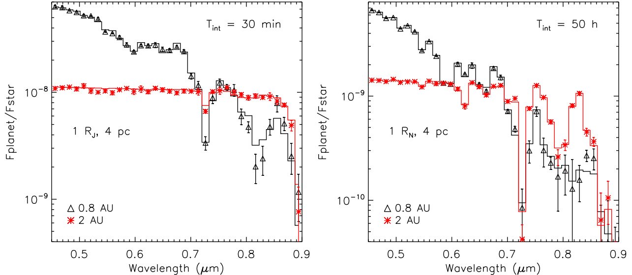
Figure 5. Simulated (symbols) and theoretical spectra of Jupiter (left) and Neptune (right) analogs for two separations to a solar-type star. For 0.8-AU planets, the atmospheric temperature is warm enough to prevent the cloud condensation and the dominant diffusion source is the Rayleigh scattering by the gas molecules. For 2-AU planets, water clouds form and flatten out the spectrum continuum.
