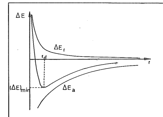
Figure 1. Potential energy curve of contact ion pair.
