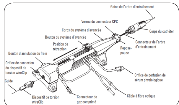
Figure 2. Le système Rotablator® (Boston Scientific).
