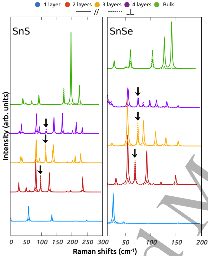
Figure 7. Simulated powder averaged Raman spectra for SnX slabs. The surface modes, indicated by a black arrow, can be related to the B_{3g} mode of SnS and SnSe bulk spectra at respectively 103 \text{cm}^{-1} and 173 \text{cm}^{-1} and shows a large parallel component compared to the other Raman active modes.
