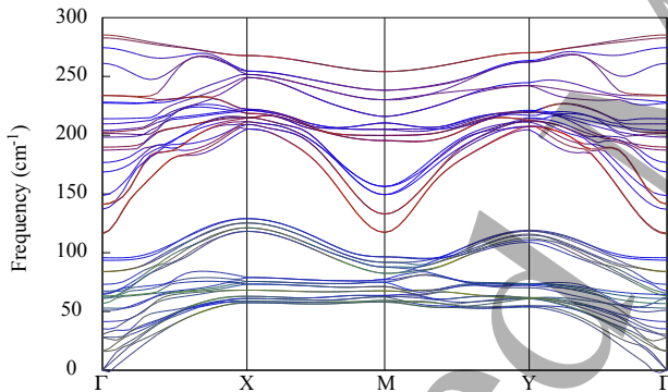
Figure 5. Phonon band structure of a 4 layer SnS slab. Colors represent the contributions of the different atoms to the modes. Sn atom in green, S atoms from inner layers in blue, S atoms of surface layers in red. A mix of these three primary colors shows modes with contributions from different atoms. We identify a surface state at 120 \text{ cm}^{-1} with lower energy than the corresponding bulk mode. Also, the two modes of highest energy involve only surface atoms.
