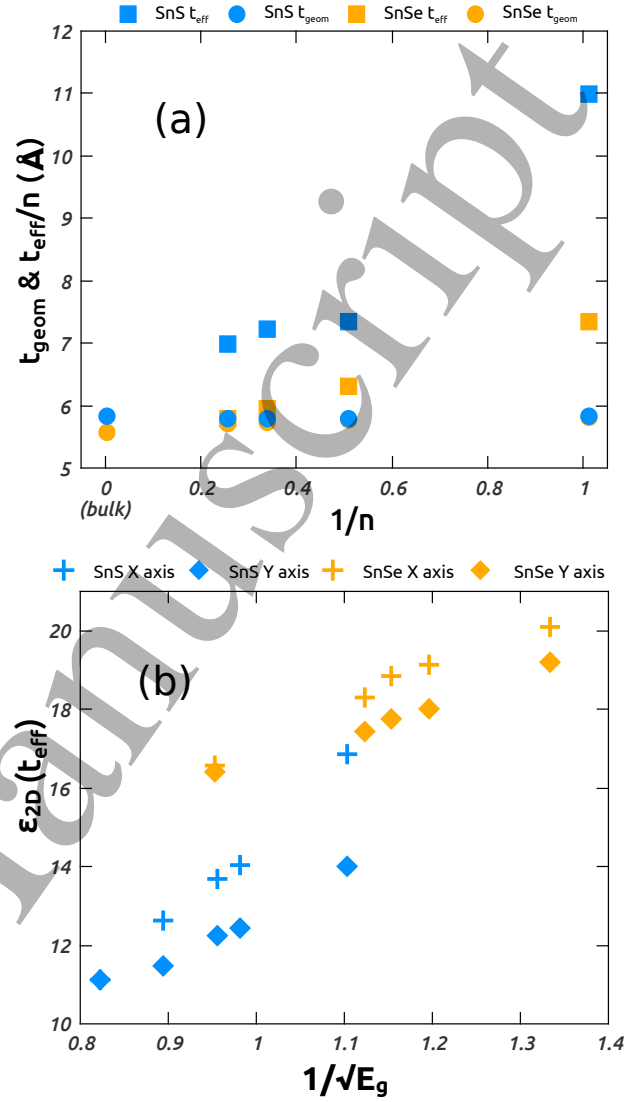
Figure 9. (a) Comparison between t_{eff} and t_{geom} . (b) Electronic dielectric constant \epsilon_{2D} rescaled with t_{eff} (note the subtle difference with Fig 8, as t_{eff} \neq t_{geom} + \text{constant} )
