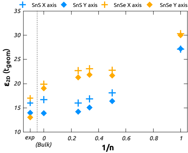
Figure 8. In-plane components of the electronic dielectric tensor for SnS and SnSe. The comparison with the experimental results of Chandrasekhar et al. [50] is shown on the left of the figure.
