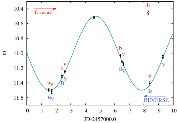
Figure 1. Single-band lightcurve simulated as m = 11.0 + 0.5 \sin(\text{JD} - 2457000.0) + \text{noise} is divided into subsamples to calculate Stetson’s variability indices (Sections 2.9 and 2.10). The arrows indicate the order in which lightcurve points are considered: first to last (subsample names in lower case) or reverse (subsample names in upper case). \Delta T_{\max} = 1 d . Dashed line is the weighted average. The weights are iteratively scaled by the factor f , see equation (14), Section 2.10. The open circle is an ‘outlier’ 1 mag brighter than it should be to follow the sine curve.
