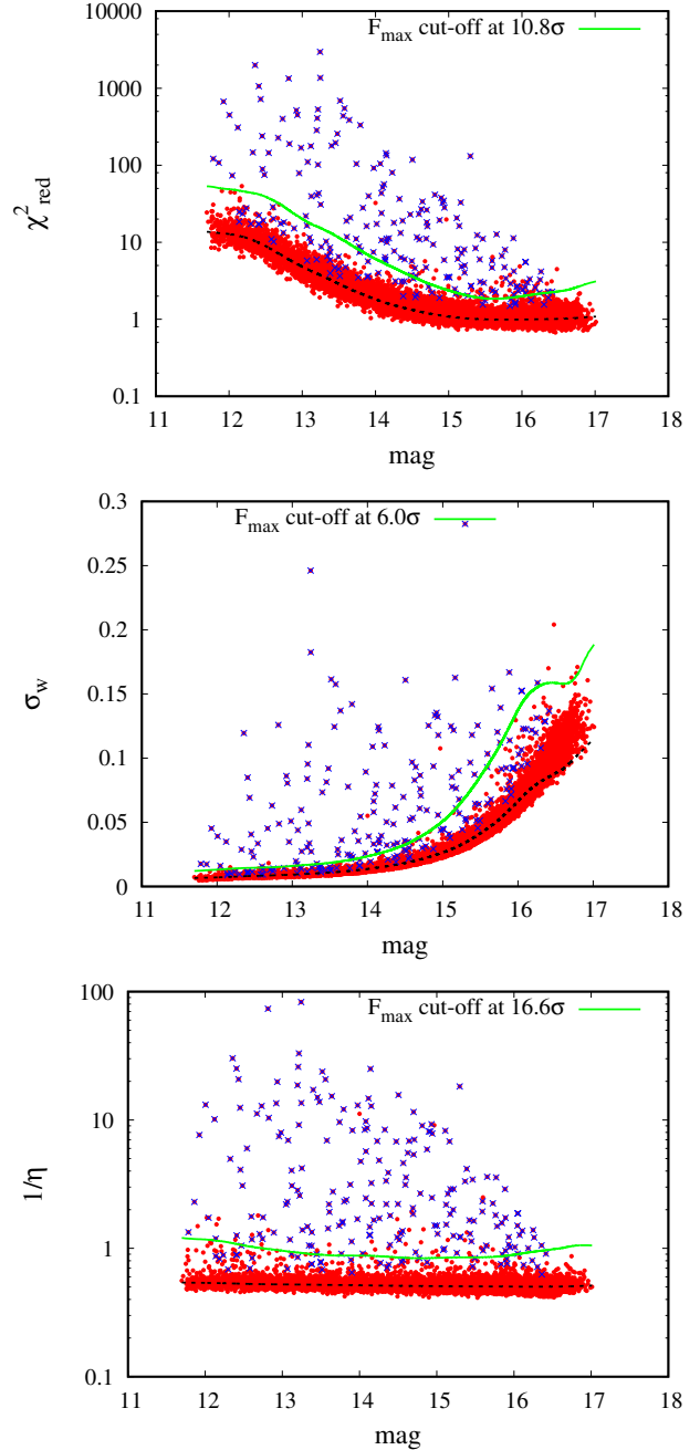
Figure 3. Variability indices \chi^2_{\text{red}} (Section 2.1), \sigma_w (Section 2.2) and 1/\eta (Section 2.15) plotted as a function of magnitude for the Krasnoyarsk data set (Section 3.2). Variable stars are marked with ‘x’. The curves represent the expected value of \chi^2_{\text{red}} , \sigma_w and 1/\eta for a given magnitude and the selection threshold corresponding to the best trade-off between the completeness and purity of the candidates list ( F_{\max} ; see Section 4, Fig. 4). The index-magnitude plots for the other indices and data sets may be found online at http://scan.sai.msu.ru/kirx/var_idx_paper/
