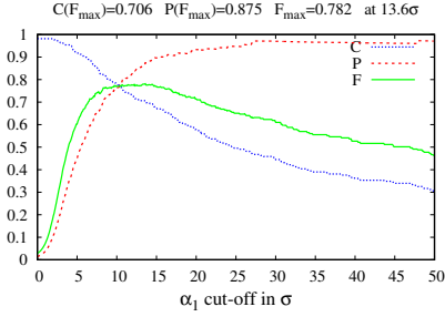
Figure 8. Variable star selection completeness ( C ), purity ( P ) and F_1 -score ( F ; see Section 4) as a function of selection threshold for the admixture coefficient \alpha_1 used as a composite variability index (Section 5.4) computed for the Kr data set (Section 3.2). Similar plots for the other data sets may be found online at http://scan.sai.msu.ru/kirx/var_idx_paper/
