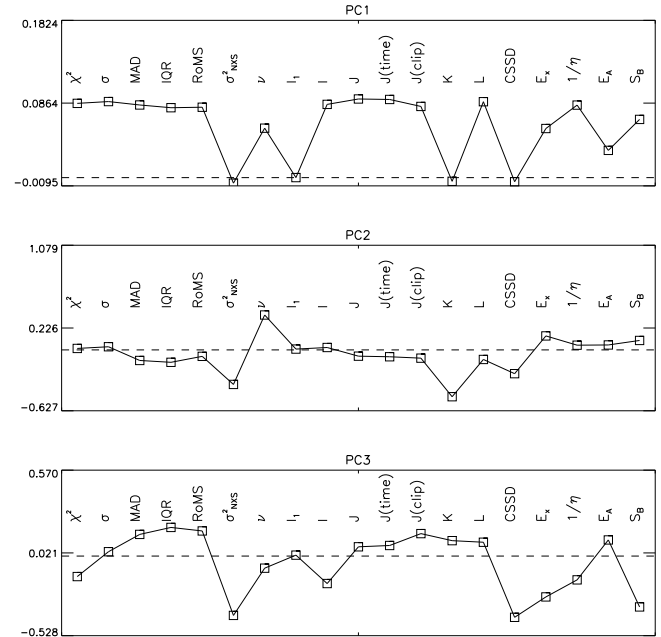
Figure 7. The first three principal components in the Kr data set (Section 3.2). The dashed line indicates zero contribution of an index to the PC. Similar plots for the other data sets may be found at http://scan.sai.msu.ru/kirx/var_idx_paper/
