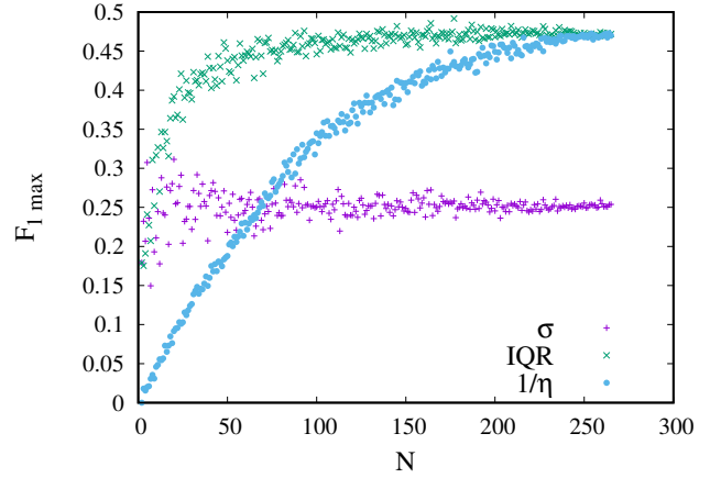
Figure 5. The F_{1\max} -score as a function of the number of lightcurve points. For each N , the random selection of N points is repeated 10 times and the median F_{1\max} value is plotted.
