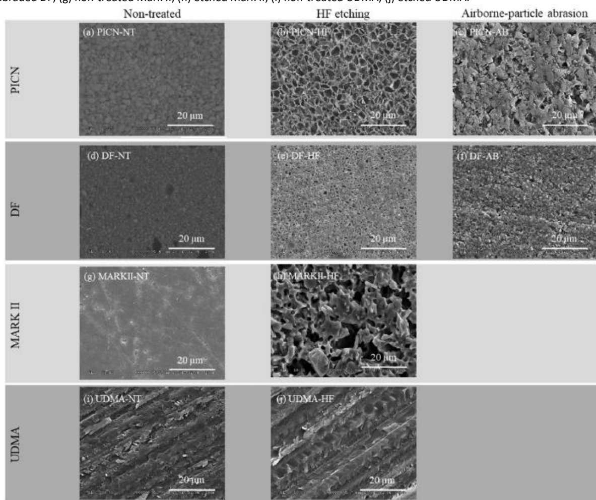
Fig. 9. Scanning electron microscopy characterization of the samples following different surface pre-treatments. (a) Non-treated PICN; (b) etched PICN; (c) airborne-particle abraded PICN; (d) Non-treated DF; (e) etched DF; (f) airborne-particle abraded DF; (g) non-treated Mark II; (h) etched Mark II; (i) non-treated UDMA; (j) etched UDMA.
