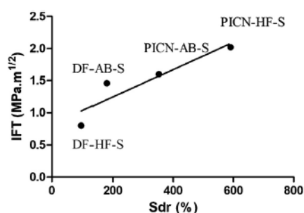
Fig. 7. Interfacial fracture toughness (IFT) versus developed interfacial area ratio (Sdr) and their correlation curve ( r^2 = 0.8411 ). Results are expressed as the means \pm SD of IFT and Sdr for the tested samples of polymer infiltrated ceramic network (PICN) materials and dispersed filler (DF). PICN-AB-S is airborne-particle abraded silanized PICN; PICN-HF-S is etched silanized PICN; DF-AB-S is airborne-particle abraded silanized dispersed fillers; DF-HF-S is etched silanized dispersed fillers.
