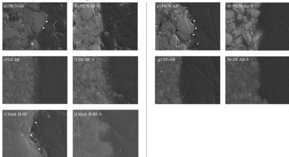
Fig. 10. Scanning electron microscopy of the cement interface with PICN, DF and Vita Mark II. The arrows are pointing at areas of incomplete wettability. (a) Etched PICN; (b) etched silanized PICN; (c) airborne-particle abraded PICN; (d) airborne-particle abraded silanized PICN; (e) etched DF; (f) etched silanized DF; (g) airborne-particle abraded DF; (h) airborne-particle abraded silanized DF; (i) etched Vita Mark II; (j) etched silanized Vita Mark II.
