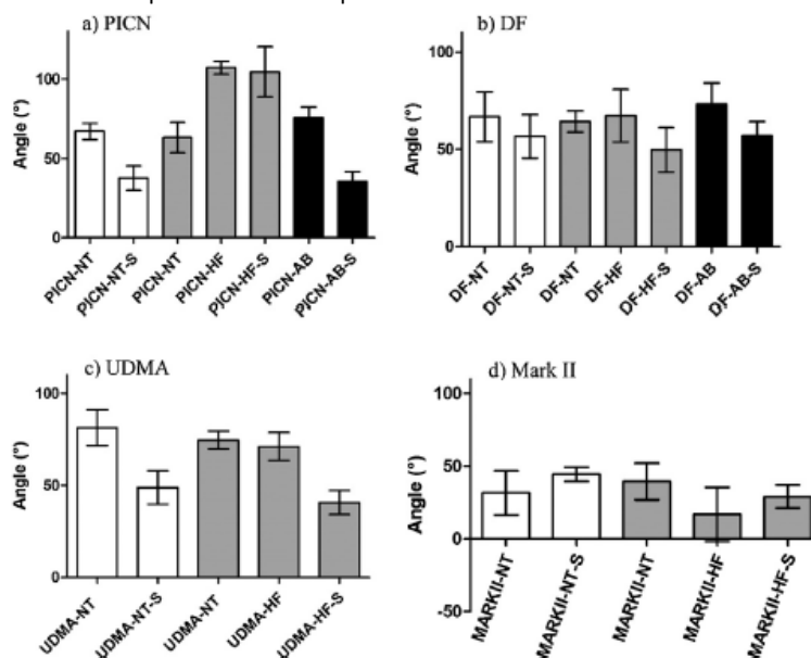
Fig. 8. Bar graphs of the results of contact angle measurements. (a) PICN; (b) DF; (c) UDMA; (d) Vita Mark II. Bars with the same color represent the same sample. Results are expressed as the means \pm SD.
