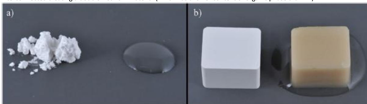
Fig. 1. (a) Fillers that are incorporated by mixing in a monomer mixture to produce a dispersed filler (DF) composite block. (b) A pre-sintered glass-ceramic scaffold infiltrated with monomer, which is secondarily polymerized under high-temperature and high-pressure to produce a polymer-infiltrated ceramic network (PICN) block. In PICN, glass-ceramic particles are interconnected creating a double-network material (which has a lower content of organic phase than DF).
