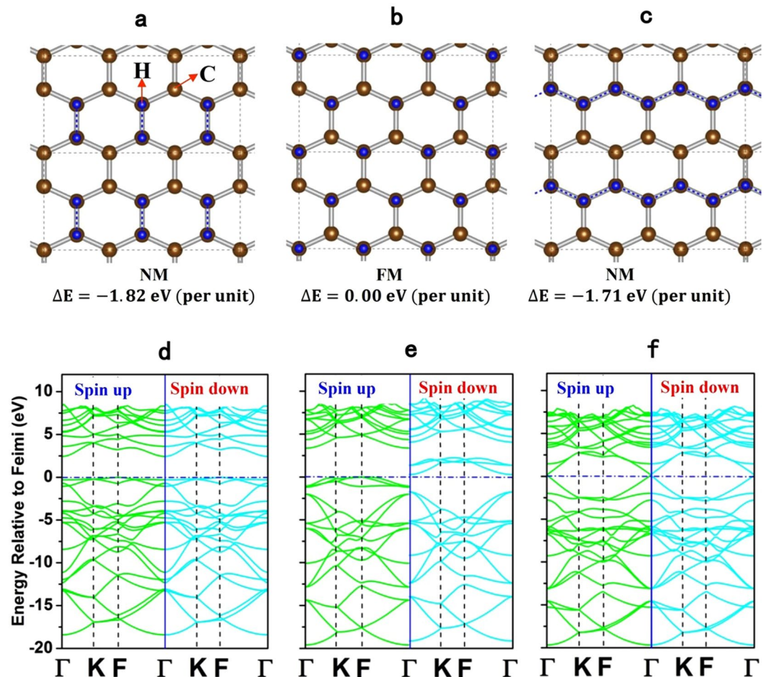
Figure 1. Schematics of the boat (a), chair (b) and zigzag (c) configurations of one-side semihydrogenated graphene. Hydrogen atoms are on the top of the 2D plane and represented by the dark blue spheres. The below corresponds to the energy band structures for the boat (d), chair (e) and zigzag (f) doping graphones, respectively. The energy band structures show that the boat, chair and zigzag doping graphones exhibit the non-magnetic semiconductor, ferromagnetic semiconductor and non-magnetic metallic properties, respectively. The boat doping graphene has the lowest energy per unit cell and is the most stable among three doping graphones.
