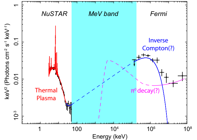
Figure 2: NuSTAR and Fermi-LAT spectra of \eta Car 20 . We need a sensitive MeV telescope to identify the signs of CR acceleration (notional \pi^0 spectrum provided for comparison.)
